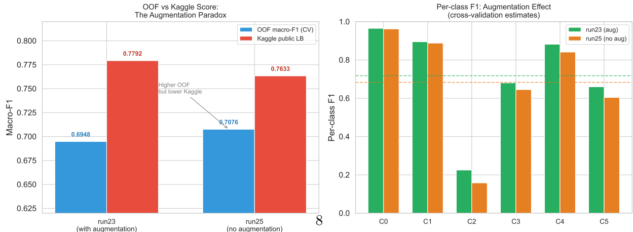
Figure 8: The augmentation paradox: 25k samples with OOF F1 (0.7076) vs 0.6948) did not
