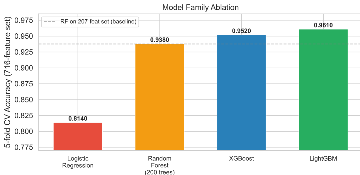
Figure 18: Model family comparison on the full feature set using 5-fold CV. LightGBM achieves the highest accuracy due to its leaf-wise tree growth strategy, which produces more expressive trees per num_leaves budget than the level-wise strategy used by XGBoost.
