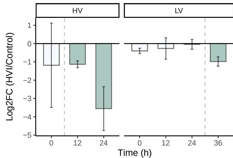
Desthiobiotin
