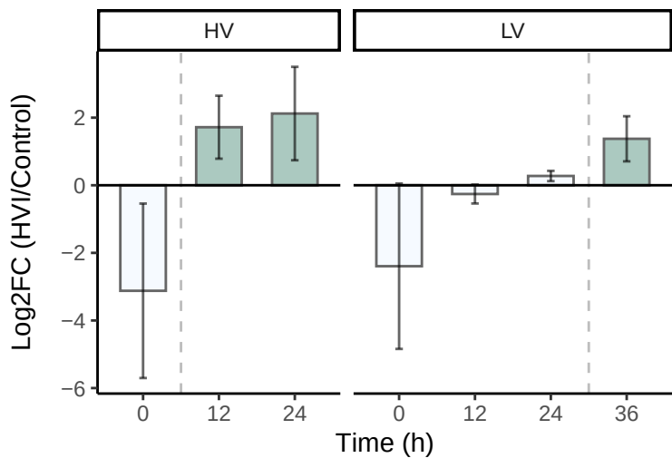
Adenine
