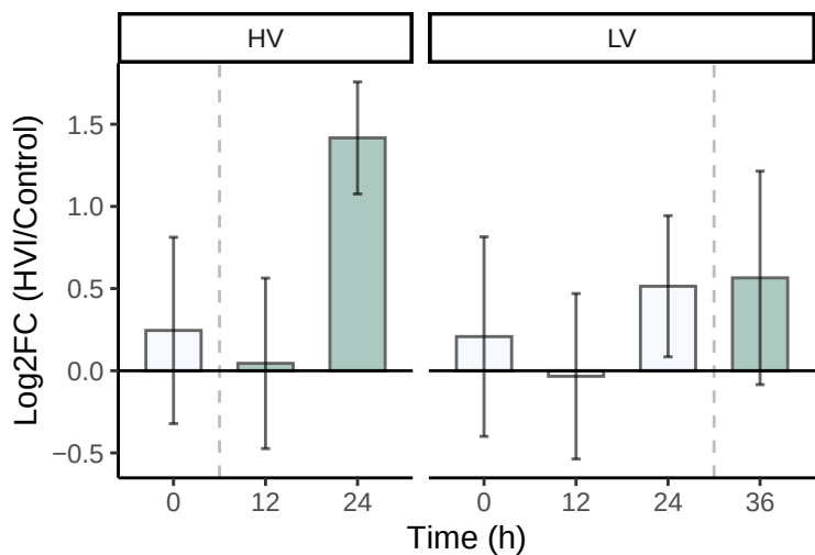
2-O-alpha-D-Glucosylglycerol
