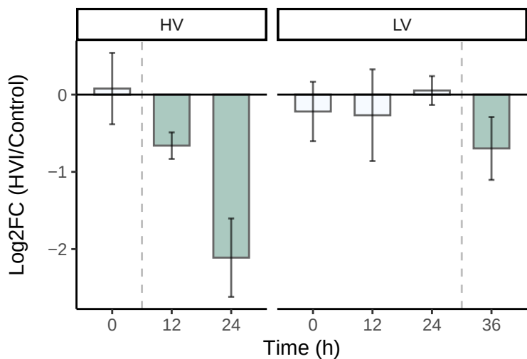
(3-Carboxypropyl)trimethylammonium
