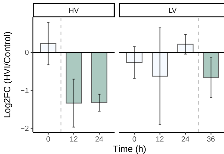
Ophthalmic acid
