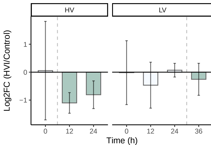
L-Lysine
