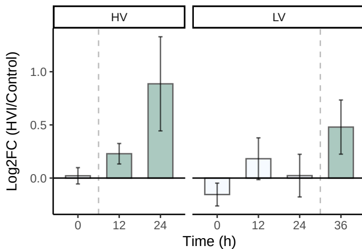
Glutathione disulfide
