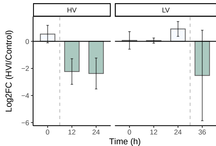
Betonicine
