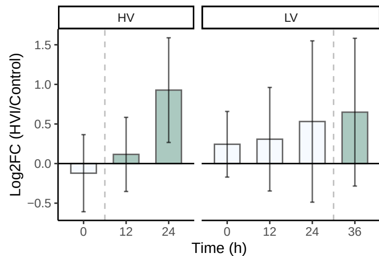
L-Aspartic acid
