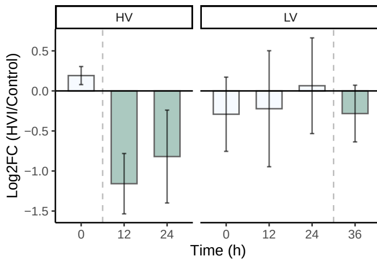
OH-Pseudocob
