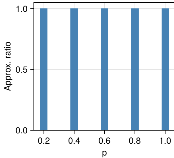
Exact Quantum
