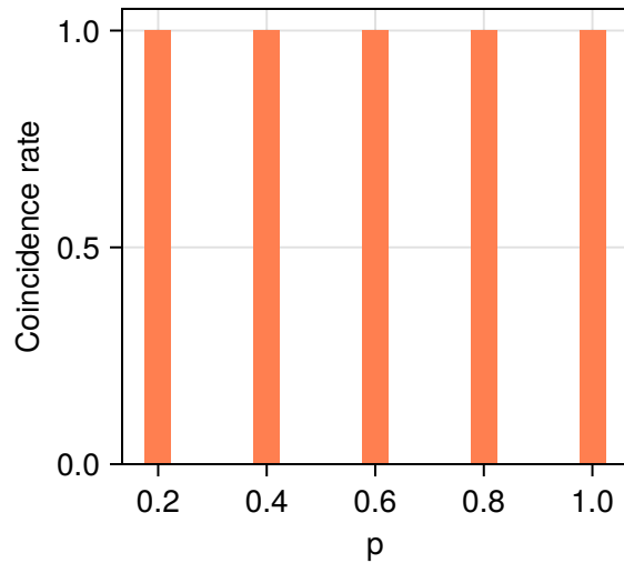
Exact Quantum
