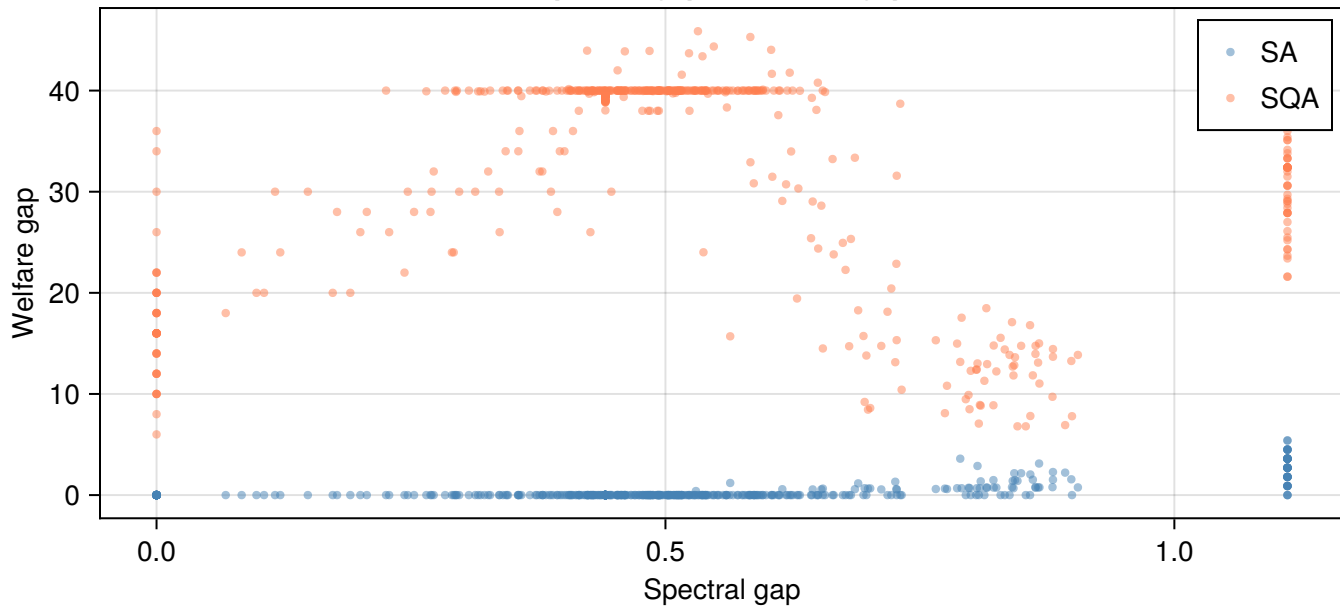
Spectral gap vs Welfare gap
