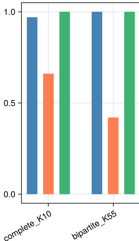
Coincidence
