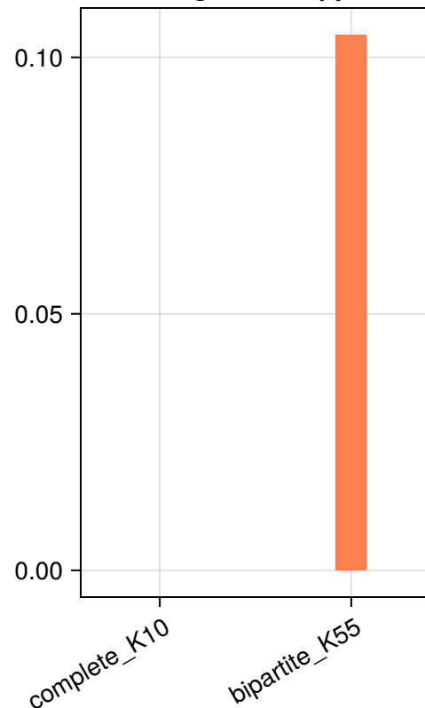
Logical entropy
