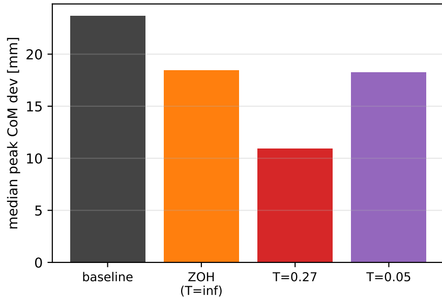
(b) Horizon-decay knee (oracle, 50 N)
