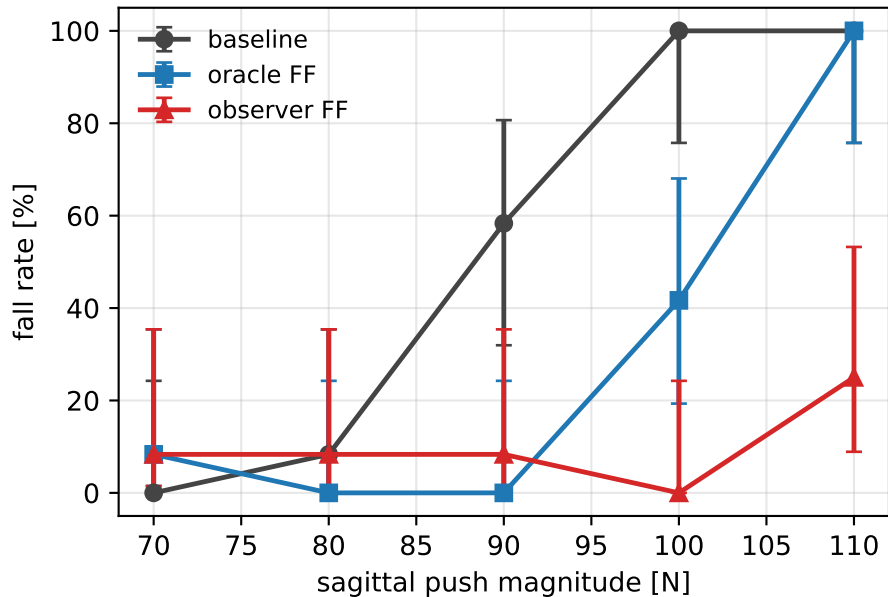
(a) Recovery vs push (sagittal, M=12)
