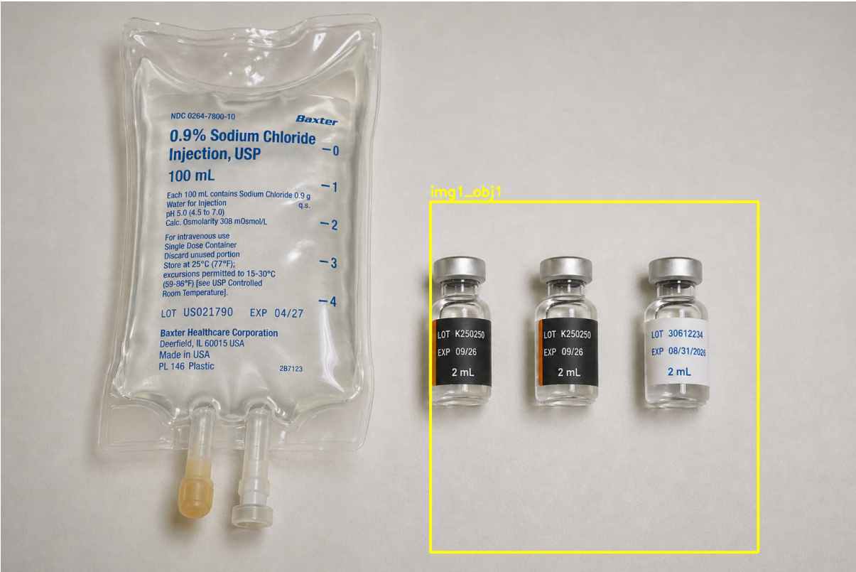
Image 1 segmentation
