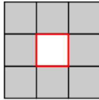
8-neighborhood
