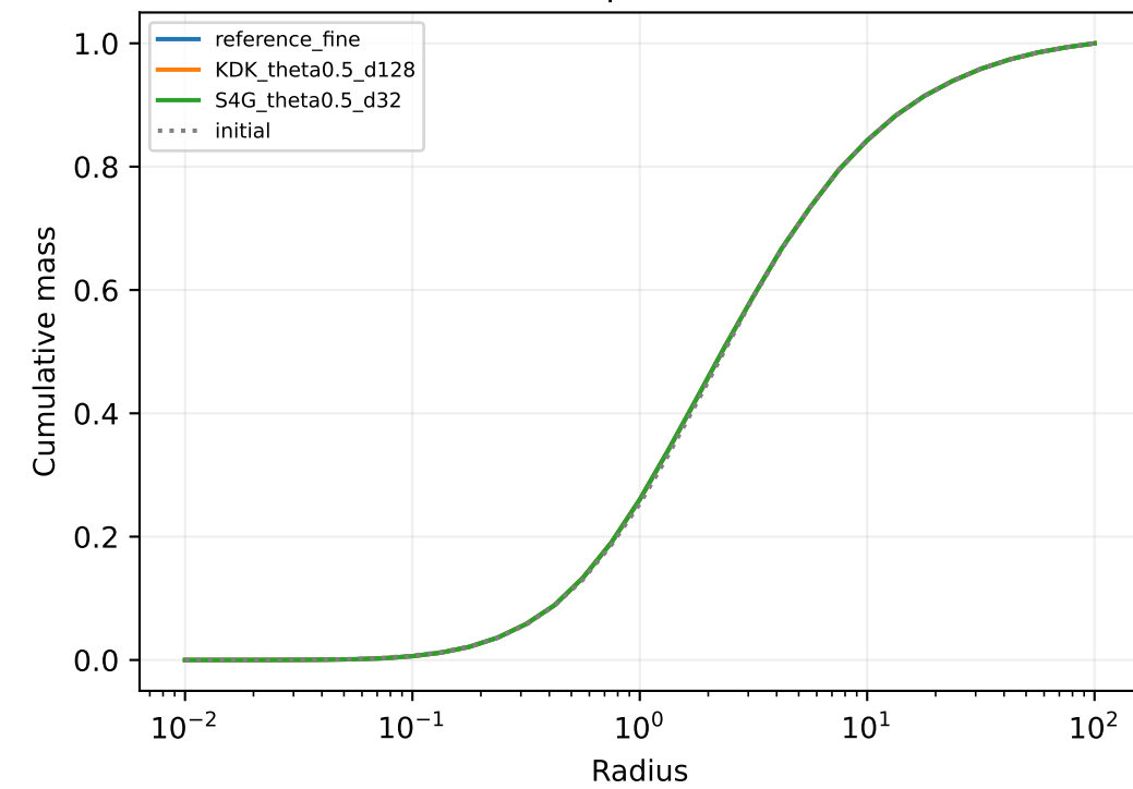
Ensemble profiles at t=6
