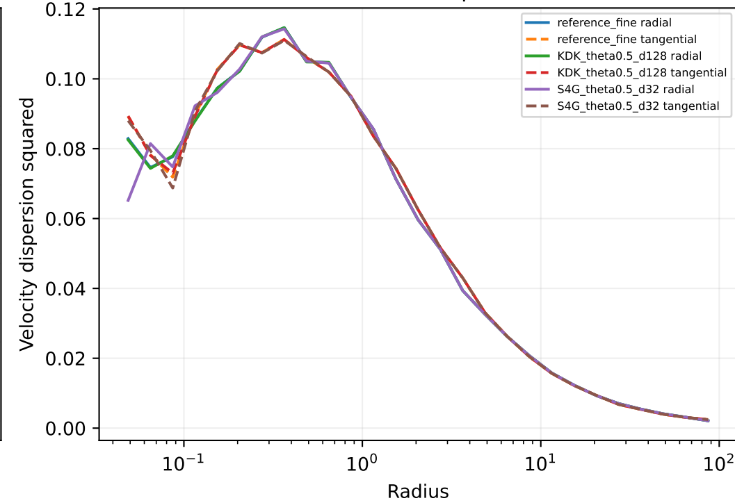
Shells with \geq 50 particles
