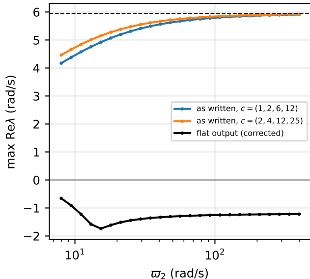
(a) closed-loop eigenvalues
