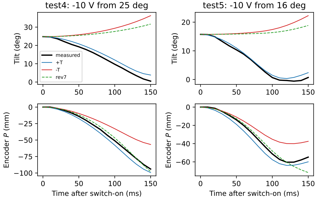
Figure 5.7: The first 150 ms after switch-on at -10 V: the on-board filtered tilt and the encoder position, and each candidate simulated open loop from rest at the logged initial tilt with the logged voltages. The filtered tilt overstates the fall during these accelerations; the gyroscope rates quoted in the text are the cleaner comparison.
