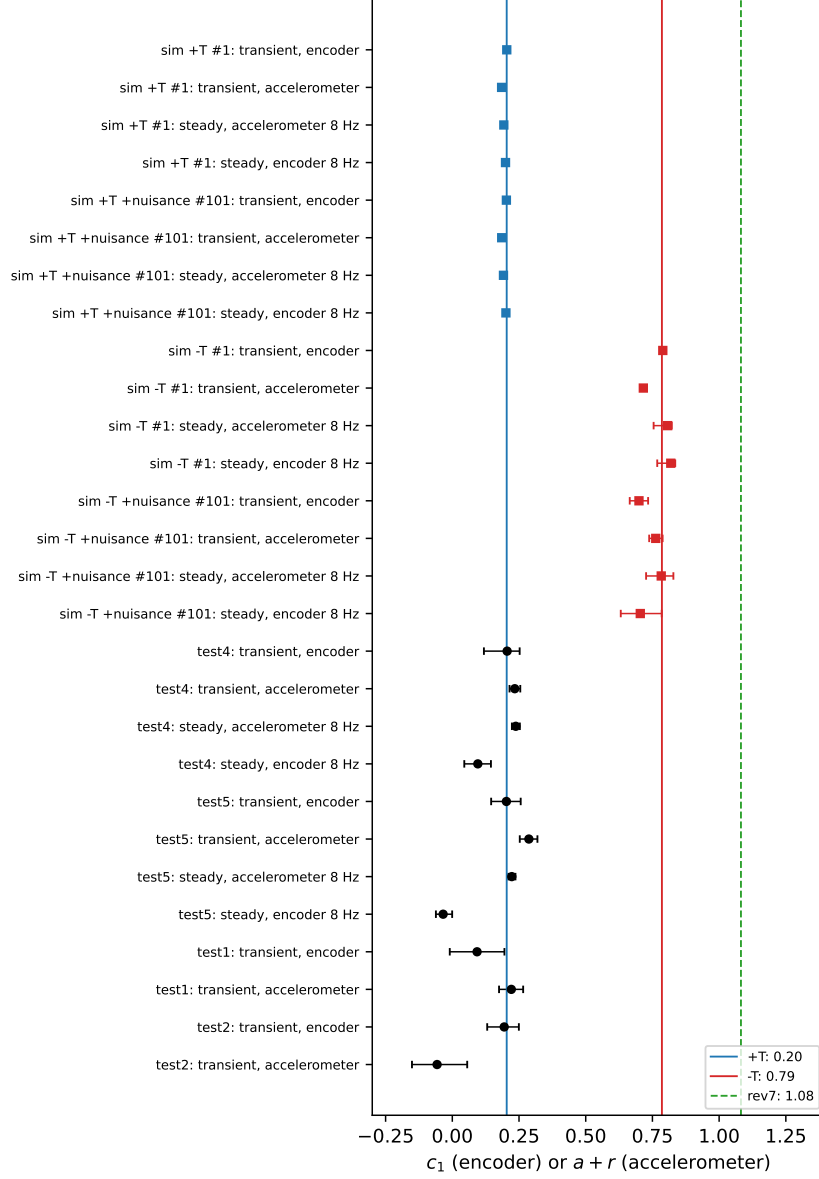
Figure 5.6: The coefficient c_1 with bootstrap intervals, from the encoder (transient and steady fits) and from the accelerometer (the transient fit a shifted by r , and the steady \ddot{\phi} coefficient shifted by r plus the IMU height): one seed of each simulated case (top) and the recorded runs (bottom). Vertical lines: M1, M2 and M3. Eight of the twelve measured intervals exclude M1; none includes M2 or M3.
