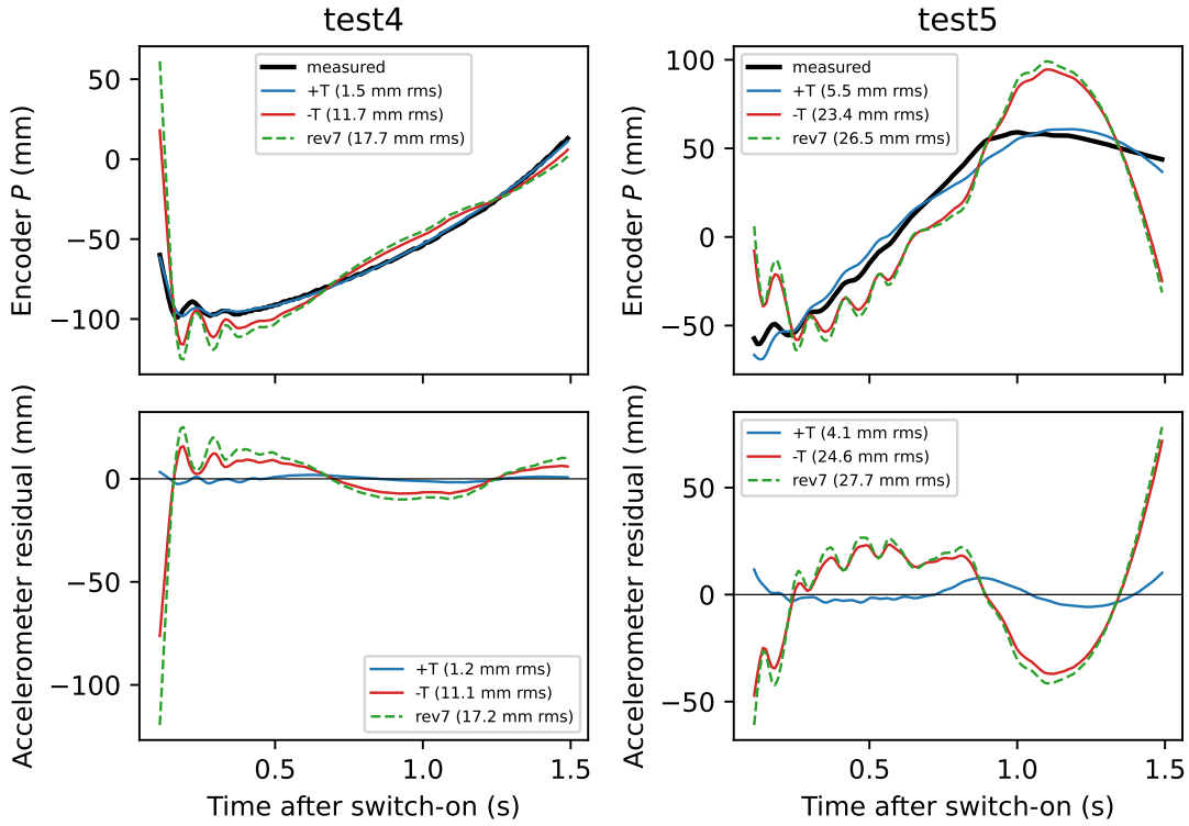
Figure 5.5: Input-free test on the switch-on transients of tests 4 and 5, plotted over 0.1 s to 1.5 s (Table 5.3 uses 0.1 s to 0.8 s; over the longer window the errors of M1 stay near 1.5 and 1.2 mm in test 4 but grow to 5.5 and 4.1 mm in test 5). Top: the logged encoder position and each candidate's prediction from the measured tilt history. Bottom: residual of the doubly integrated accelerometer against each candidate.
