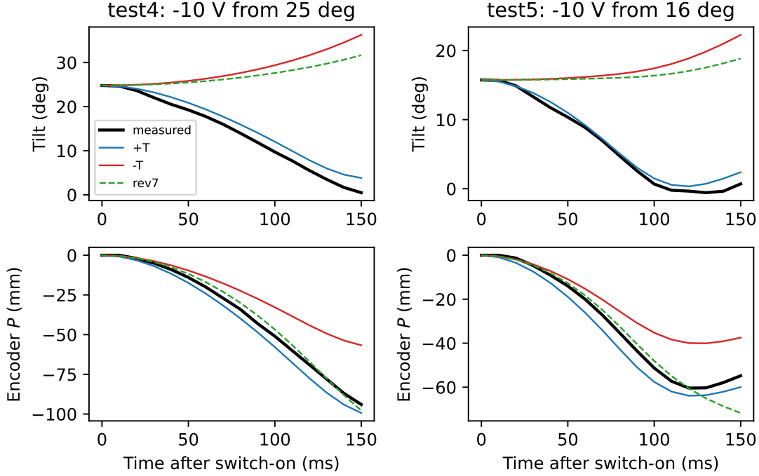
Figure 5.7: The first 150 ms after switch-on at -10 V: measured tilt and encoder position, and each candidate simulated open loop from the logged initial state with the logged voltages.
