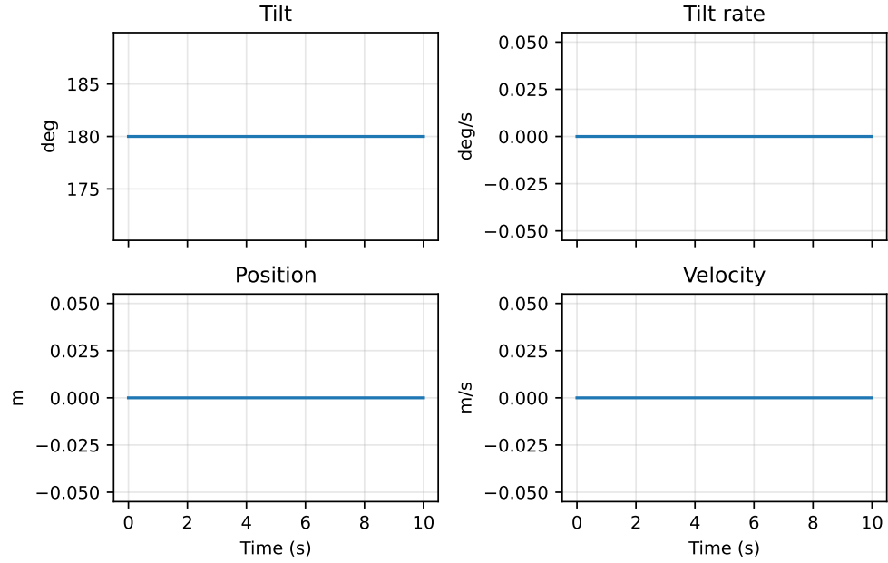
Figure 5.3: Uncontrolled response from \theta = 180^\circ (model M1).
