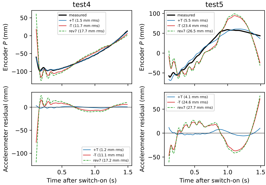
Figure 5.5: Input-free test on the switch-on transients of tests 4 and 5. Top: the logged encoder position and each candidate's prediction from the measured tilt history. Bottom: residual of the doubly integrated accelerometer against each candidate.
