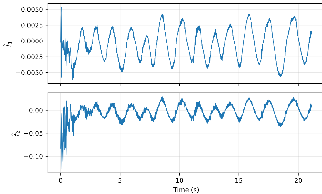
Figure 8.10: Hardware test: DMSO uncertainty estimates.
