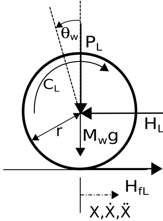
Figure 5.1: Left wheel free body diagram.
