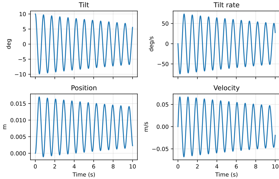
Figure 5.4: Uncontrolled response from \theta = 10^\circ (model M1).
