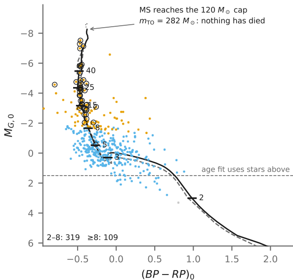
Cyg OB2-C PARSEC 2.52 Myr · MIST 3.16 Myr
