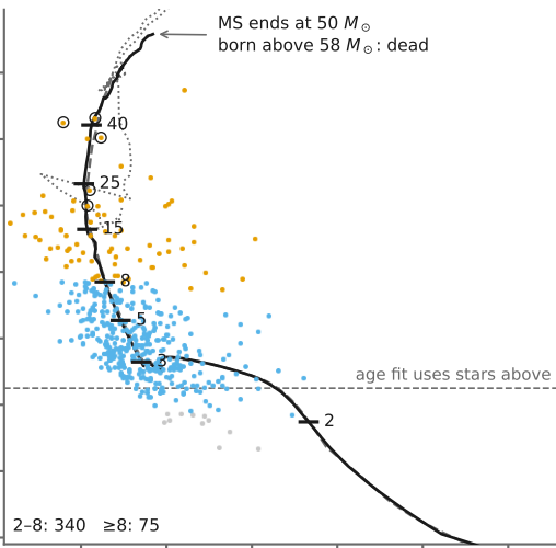
Cyg OB2-B PARSEC 4.09 Myr · MIST 4.01 Myr
