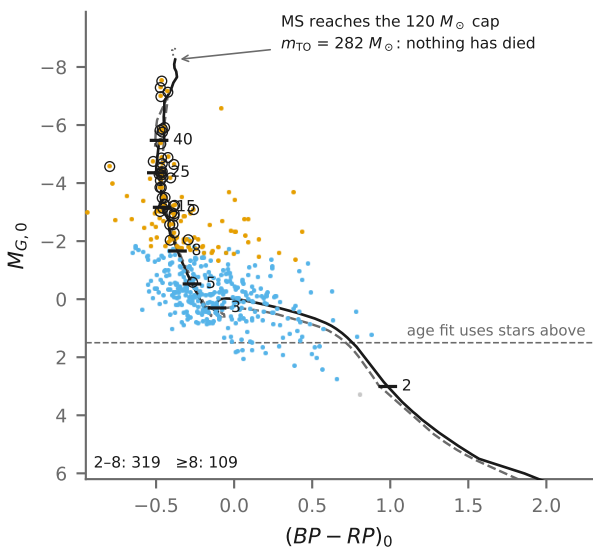
Cyg OB2-C PARSEC 2.52 Myr · MIST 3.16 Myr
