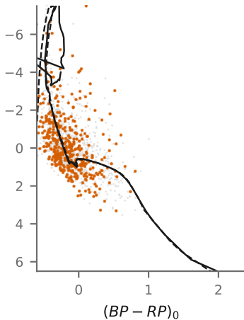
Cyg OB2-B 4.09 Myr
