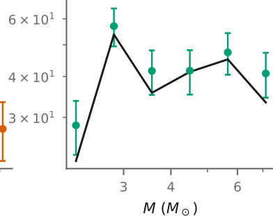
Cyg OB2-C max |r| = 1.34
