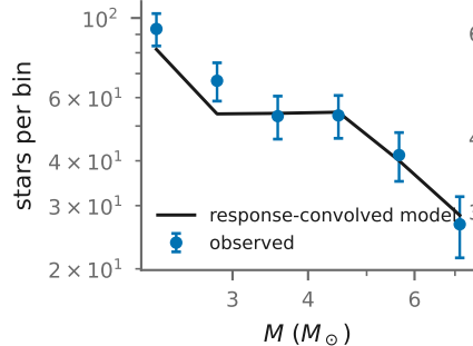
Cyg OB2-A max |r| = 1.74
