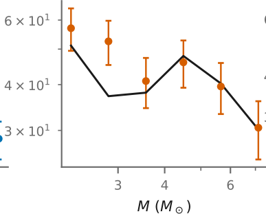
Cyg OB2-B max |r| = 2.51
