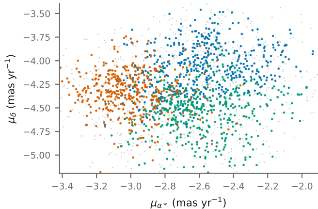
subgroups from (l, b, \mu_{\alpha^*}, \mu_{\delta}) only
