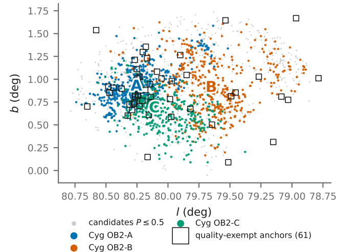
selected on (l, b, \varpi, \mu_{\alpha^*}, \mu_{\delta})
