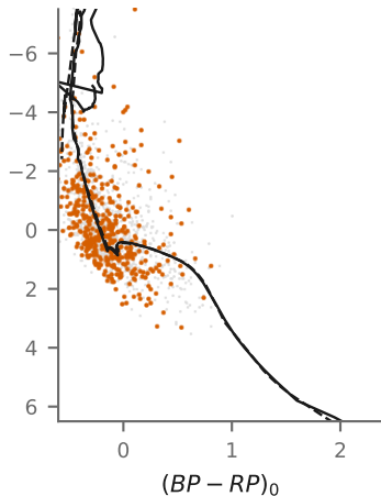
Cyg OB2-B 3.70 Myr
