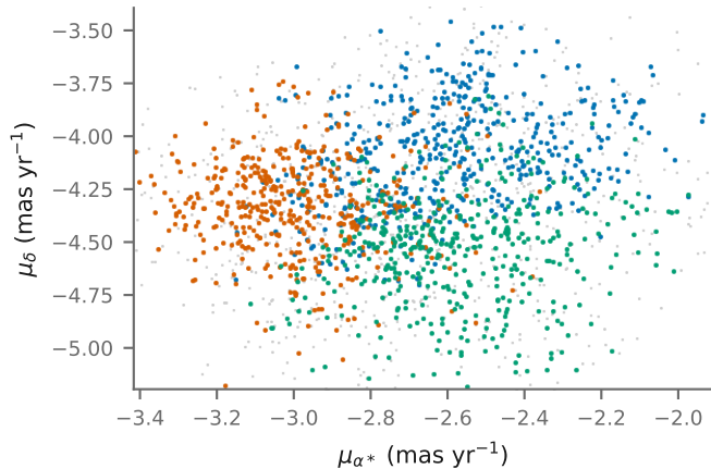
subgroups from (l, b, \mu_{\alpha^*}, \mu_{\delta}) only
