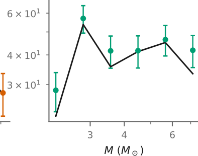
Cyg OB2-C max |r| = 1.48
