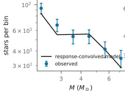
Cyg OB2-A max |r| = 1.56
