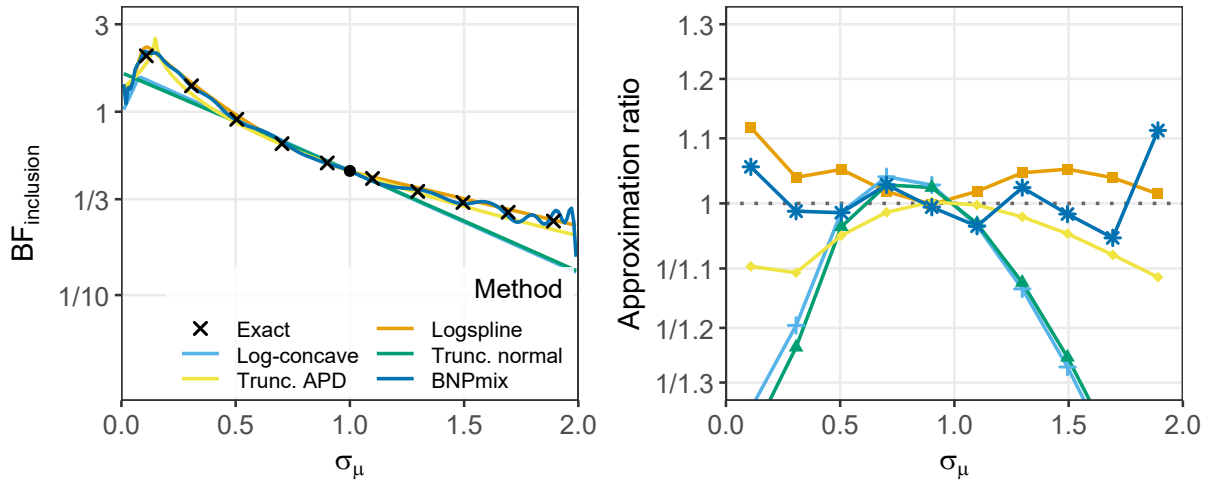
Figure 9: Sensitivity analysis for the robust Bayesian meta-analysis applied to the Bem (2011) data: reduced appendix display of the supplementary density estimators. Left panel: inclusion Bayes factor BF_{\text{incl}} as a function of the prior standard deviation for the overall effect, \sigma_\mu ; colored lines show logspline density estimation, the log-concave maximum likelihood estimator, the truncated normal approximation, the truncated asymmetric power distribution (APD), and the Bayesian nonparametric mixture estimator from BNPmix. Right panel: approximation ratio BF_{\text{approx}}/BF_{\text{exact}} at the validation points. The product-space approach is used throughout; the filled circle marks the anchor at \sigma_\mu = 1 , and crosses show validation refits of the full 36-model robust Bayesian meta-analysis obtained by bridge sampling.
