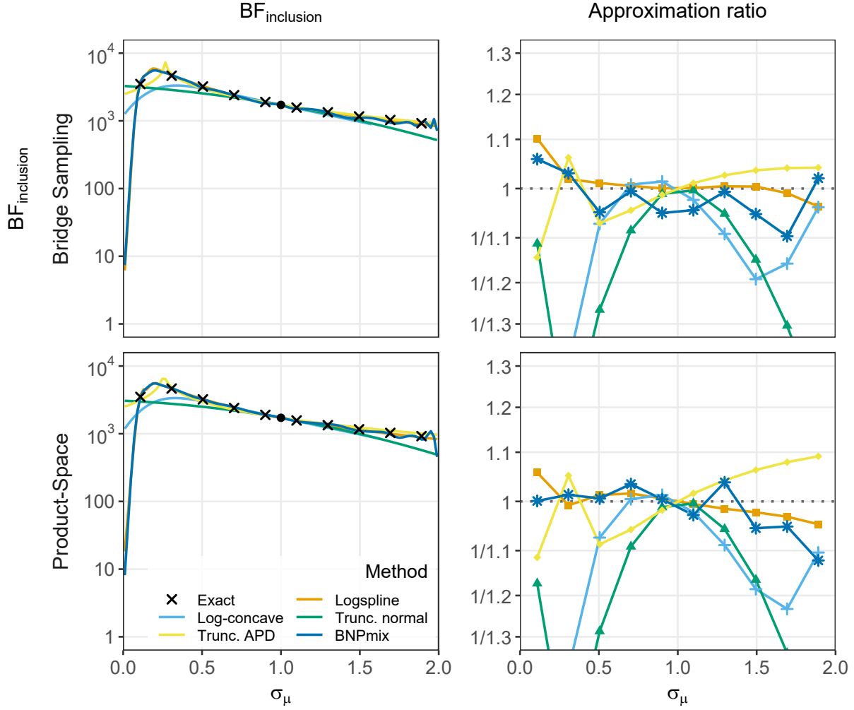
Figure 8: Sensitivity analysis for the Bayesian model-averaged meta-analysis applied to the Bem (2011) data: reduced appendix display of the supplementary density estimators. Rows correspond to the two encompassing strategies (top: bridge sampling; bottom: product-space). Left column: inclusion Bayes factor BF_{\text{incl}} as a function of the prior standard deviation for the overall effect, \sigma_\mu ; colored lines show logspline density estimation, the log-concave maximum likelihood estimator, the truncated normal approximation, the truncated asymmetric power distribution (APD), and the Bayesian nonparametric mixture estimator from BNPmix. Right column: approximation ratio BF_{\text{approx}}/BF_{\text{exact}} at the validation points. Filled circles mark the anchor at \sigma_\mu = 1 ; crosses show validation refits of the full Bayesian model-averaged meta-analysis obtained by bridge sampling.
