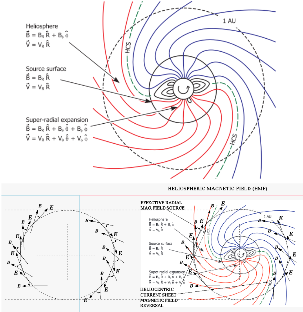
Figure 2: Top: Copied from Owens and Forsythe[2], as follows: “A sketch of the steady-state solar magnetic field in the ecliptic plane. Close to the sun, in a spatial region approximately bounding the solar corona, the magnetic field dominates the plasma flow and undergoes significant non-radial (or super-radial) expansion with height. At the source surface, typically taken to be a few solar-radii, the pressure-driven expansion of the solar wind dominates and both the field and flow become purely radial. In the heliosphere, rotation of the heliospheric magnetic field (HMF) footprints within a radial solar wind flow generates an azimuthal component of the HMF, B_\phi , leading to a spiral geometry. Regions of opposite HMF polarity, shown as red and blue, lines, are separated by the heliospheric current sheet (HCS), shown as the green dashed line. Image adopted originally from Schatten, Wilcox, and Ness. Bottom: Embellishments of the top figure. The figure on the right shows the local electric and magnetic field directions, illustrating, for example, the Heliocentric current sheet (HCS) and its reversal. The figure on the left defines the Parker angle \theta_P orienting the B -field lines relative to the effective radial magnetic field source and demonstrating its constancy.”
