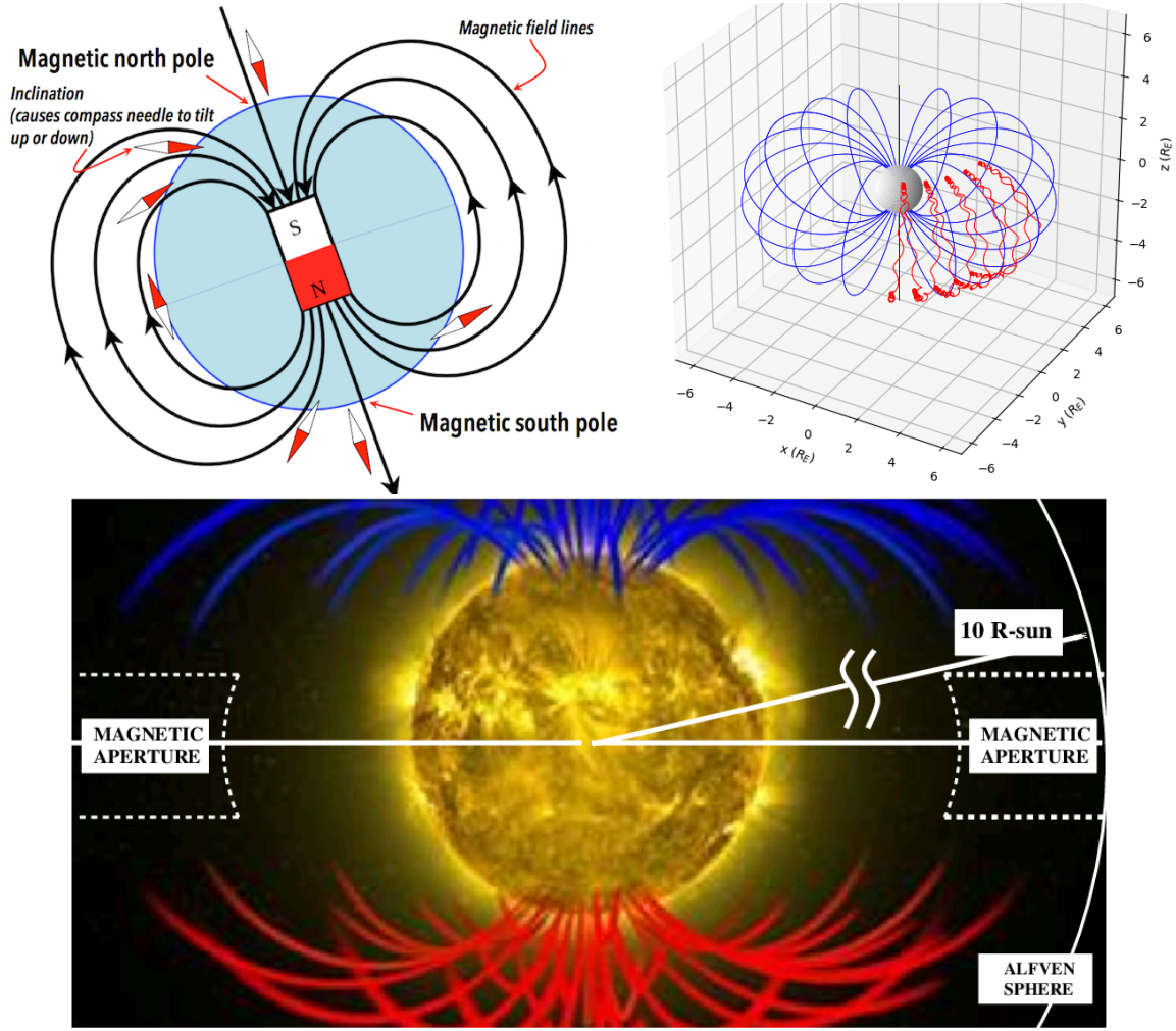
Figure 3: Top left: Magnetic dipole field pattern. Top right: Perspective view of dipole field pattern. 16 field lines are shown (actually +1, including the straight line from observer's view point). Bottom: 2025 image shows magnetic fields radiating from the sun's poles. Courtesy of NASA's Goddard Space Flight Center. Superimposed is the outline of the aperture of the sun as a particle accelerator. Interpolated onto the photograph are outlines of a virtual vacuum chamber for the sun as particle accelerator. Also indicated, at approximately 15 times the sun's radius, is the Alfvén radius, which figures prominently in the sun's injection, acceleration, and extraction processes.
