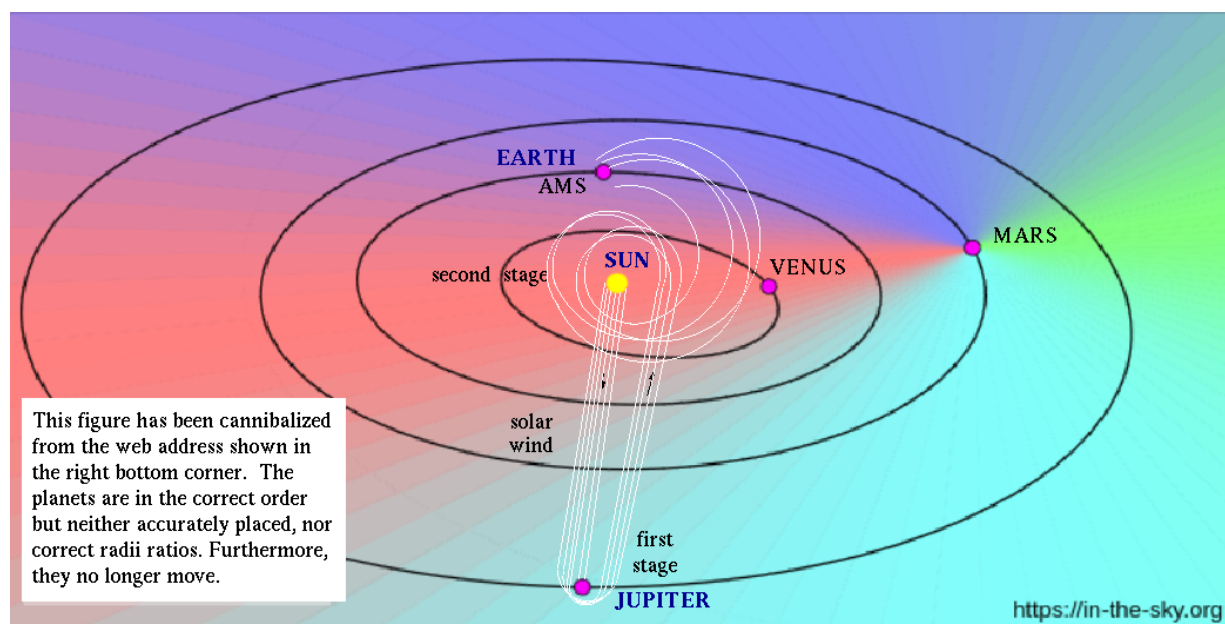
Figure 10: Artist's conception of two stage "Double-Slingshot" solar system production of cosmic rays, impinging, for example, upon the Alpha Magnetic Spectrometer (AMS) detector[3] aboard the International Space Station (ISS). As indicated in the corner note, planetary distances from the sun are much distorted. Mainly, the radius of Jupiter has been reduced, relative to the other planets, including earth, by roughly a factor of two. Slingshots first around Jupiter, then around the sun, produce acceleration factors discussed in Section (2). Of the six orbits shown leaving the sun towards Jupiter, two could potentially be detected near Earth by the AMS detector.
