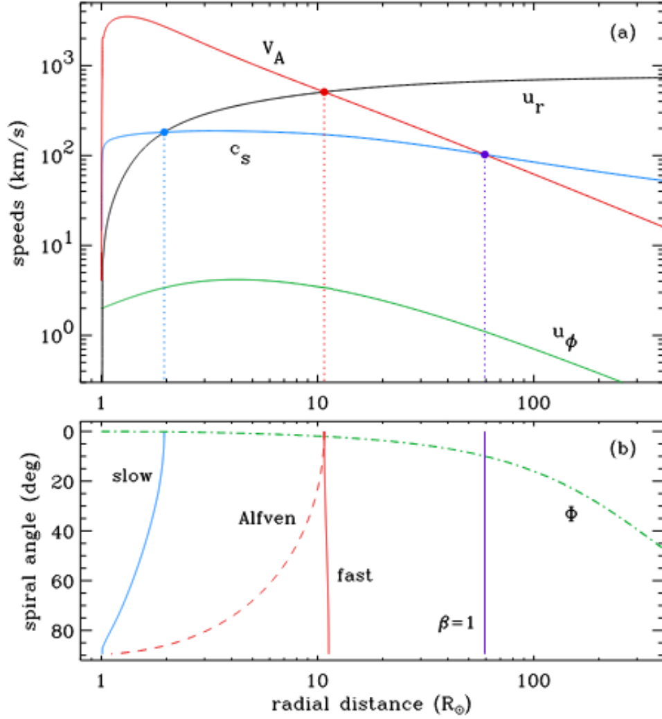
Example one-dimensional solar-wind model, with quantities plotted vs. heliocentric radial distance r , in units of solar radii R_{\odot} : (a) radial outflow speed (black), sound speed (blue), Alfvén speed V_{A,r} = B_r/(4\pi\rho)^{1/2} (red), and azimuthal flow speed (green); (b) locations of MHD critical points shown with respect to both r and the Parker spiral angle \Phi (red and blue curves), plotted alongside the self-consistent \Phi(r) for the Weber and Davis (1967) model (green dot-dashed curve). In both panels, purple denotes the \beta = 1 surface (see text).
