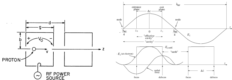
Figure 7: Copied from Loew and Talman, the left figure shows one of the many RF-cavity accelerating cells of an Alvarez linac needed to produce a “slow” (meaning slower than the speed of light) electromagnetic traveling wave. to produce the desired wave speed, such that a moving proton is always “on crest”. The right figure resembles Figure 12.1 in Kulsrud’s “Plasma Physics for Astrophysics book”.
