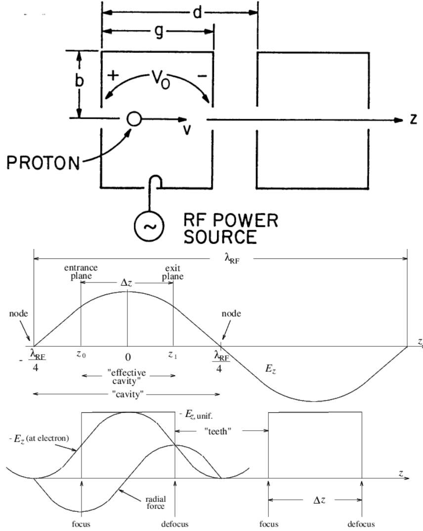
Figure 18: Copied from Loew and Talman,[23] the upper figure shows one of the many RF-cavity accelerating cells of an Alvarez linac needed to produce a “slow” (meaning slower than the speed of light) electromagnetic traveling wave. Individual cells, though seemingly independent, are phased to produce the desired wave speed, for example such that a moving proton is always “on crest”. The lower figure resembles Figure 12.1 in the Kudsrud book[22] which shows plasma fields capable of accelerating cosmic rays in galactic magneto-hydrodynamic Alfvén waves. This figure, applicable to cells in an Alvarez linac, models a proton’s instantaneous position and replacement of actual accelerating field by a train of uniform field “teeth” of thickness \Delta z \simeq \lambda_{RF}/4 . Any radial force is modeled by delta functions at entrances and exits.
