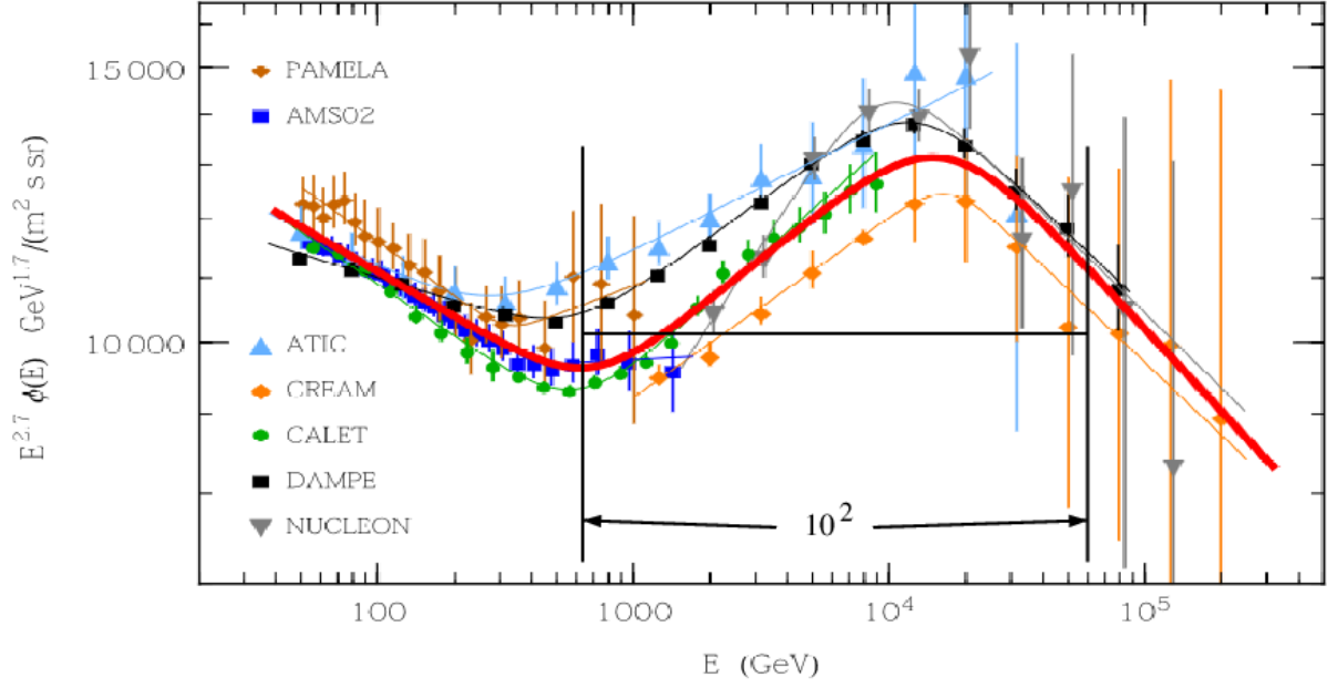
Figure 12: This figure has been copied from Lipari and Vernetto[8]. This data shows that all seven experiments on the ISS were subjected to the same impulse, or that all protons were subjected to the same impulse when near the sun. In the present paper this is interpreted as acceleration of protons from 600 GeV, to 60,000 GeV, while briefly circulating around the sun.
