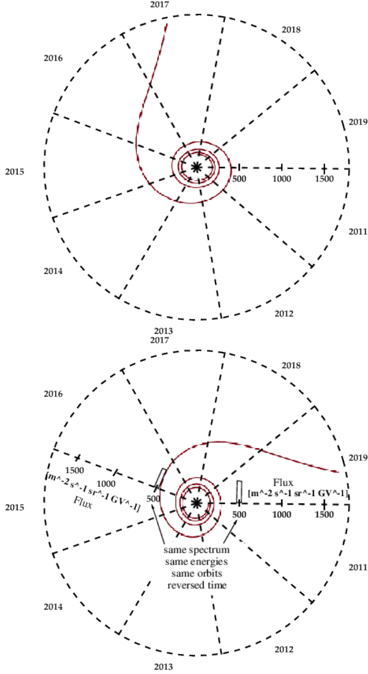
Figure 14: Top: Calculated (pseudo)-orbit for a proton departing from AMS for the sun in mid 2017. Bottom: Calculated (pseudo)-orbit (assuming negligible magnetic field in both cases) for proton departing from the sun for AMS in mid 2019.
