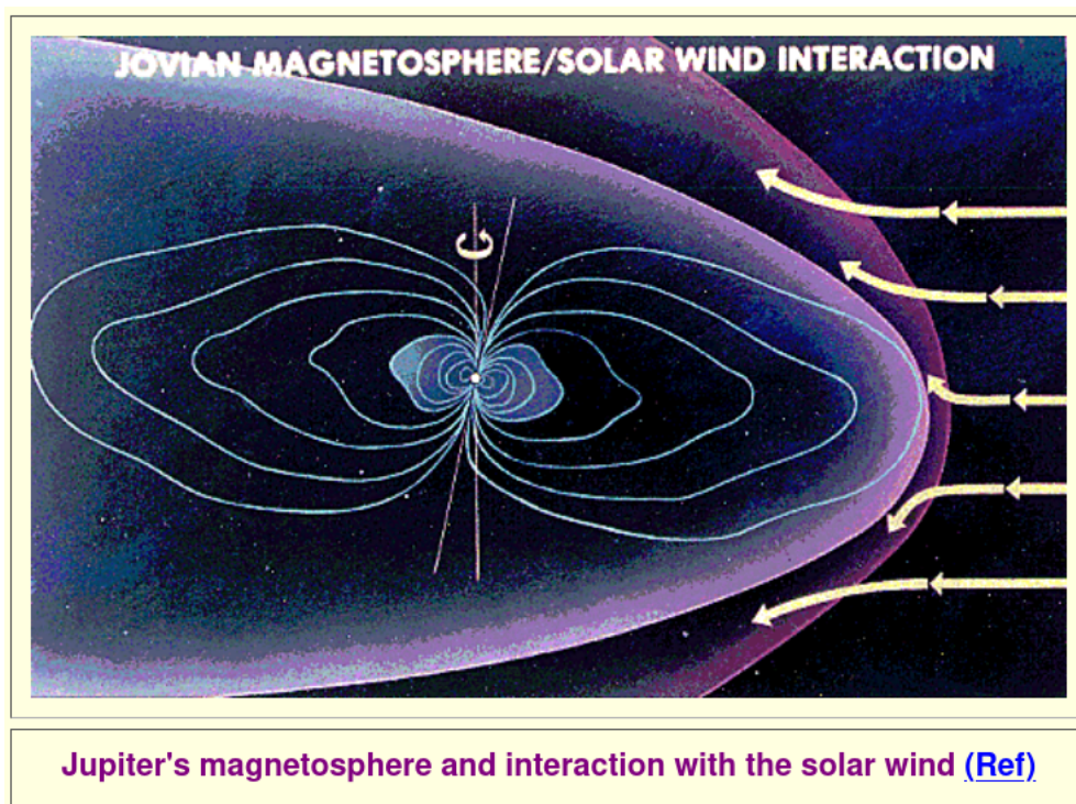
Figure 6: Jupiter magnetic field contours, copied from reference [13].
