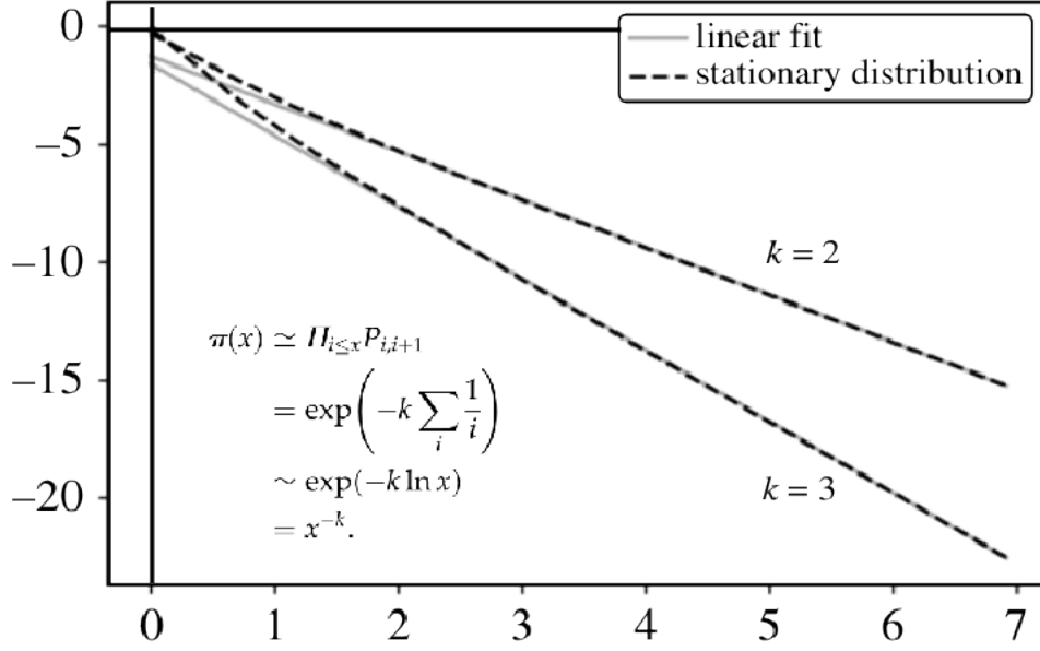
Figure 16: Copied from Roman and Bartoletti [11] “A master equation for power laws”, this figure shows how an iterated Markov stochastic distribution with one parameter (in this case, k=2 ) can match a different Markov process with parameter ( k=3 ). Applied to our case, periodic perturbation of one Markov process, over a large (but finite) range of abscissas, can be accurately matched to a different Markov process. As explained in the text, this could account for the kinks in Figure (10), while continuing to treat the overall process as Markovian. In this way one can understand (as mathematics) why there need to be kinks at low energy but (as physics) there has to be an explanation for all fits having exactly the same slopes in the high energy limit, as shown in Figure (10).
