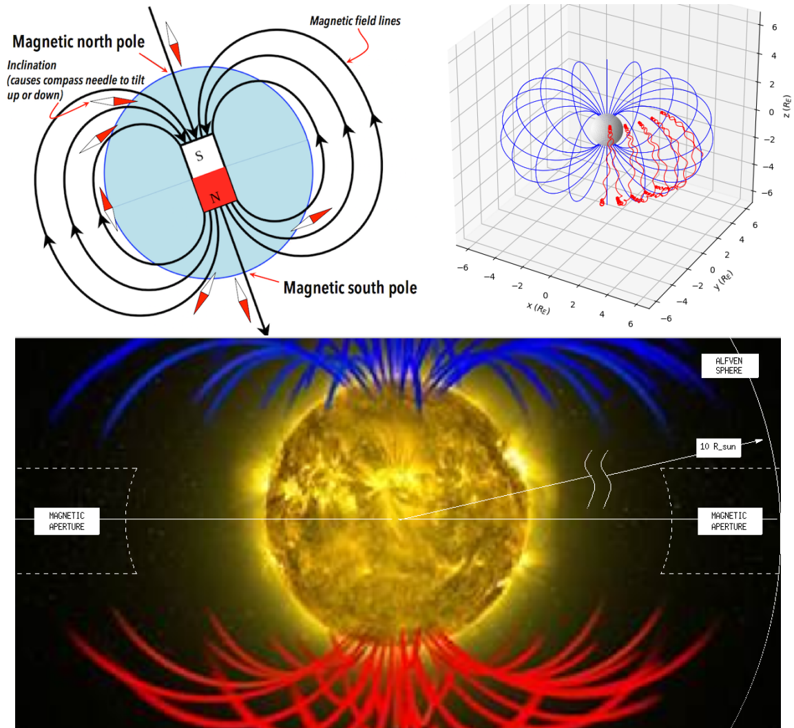
Figure 3: Top left: Magnetic dipole field pattern. Top right: Perspective view of dipole field pattern. 16 field lines are shown (actually +1, including the straight line from observer's view point). Bottom: 2025 image shows magnetic fields radiating from the sun's poles. Courtesy of NASA's Goddard Space Flight Center. Superimposed is the outline of the aperture of the sun as a particle accelerator. Interpolated onto the photograph are outlines of a virtual vacuum chamber for the sun as particle accelerator. Also indicated, at approximately 15 times the sun's radius, is the Alfvén radius, which figures prominently in the sun's injection, acceleration, and extraction processes.
