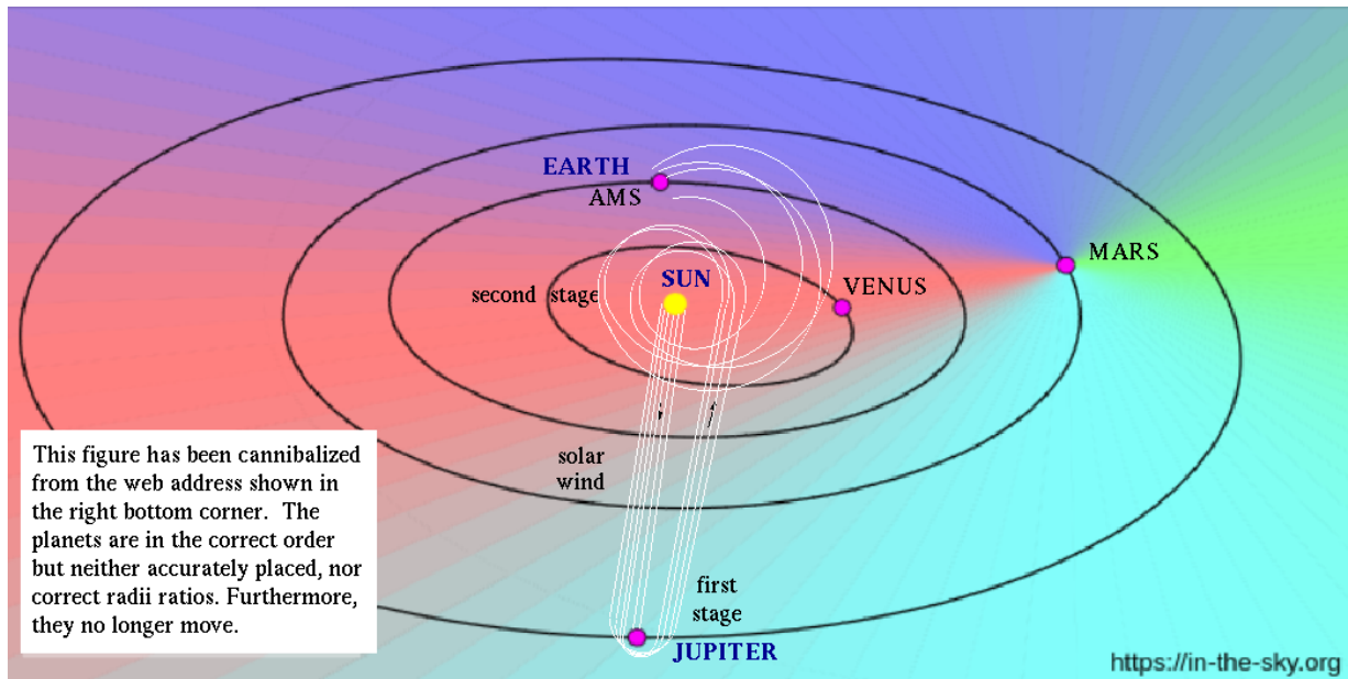
Figure 9: Artist's conception of two stage "Double-Slingshot" solar system production of cosmic rays, impinging, for example, upon the Alpha Magnetic Spectrometer (AMS) detector[10] aboard the International Space Station (ISS). As indicated in the corner note, planetary distances from the sun are much distorted. Mainly, the radius of Jupiter has been reduced, relative to the other planets, including earth, by roughly a factor of two. Slingshots first around Jupiter, then around the sun, produce acceleration factors discussed in Section (2). Of the six orbits shown leaving the sun towards Jupiter, two could potentially be detected near Earth by the AMS detector.
