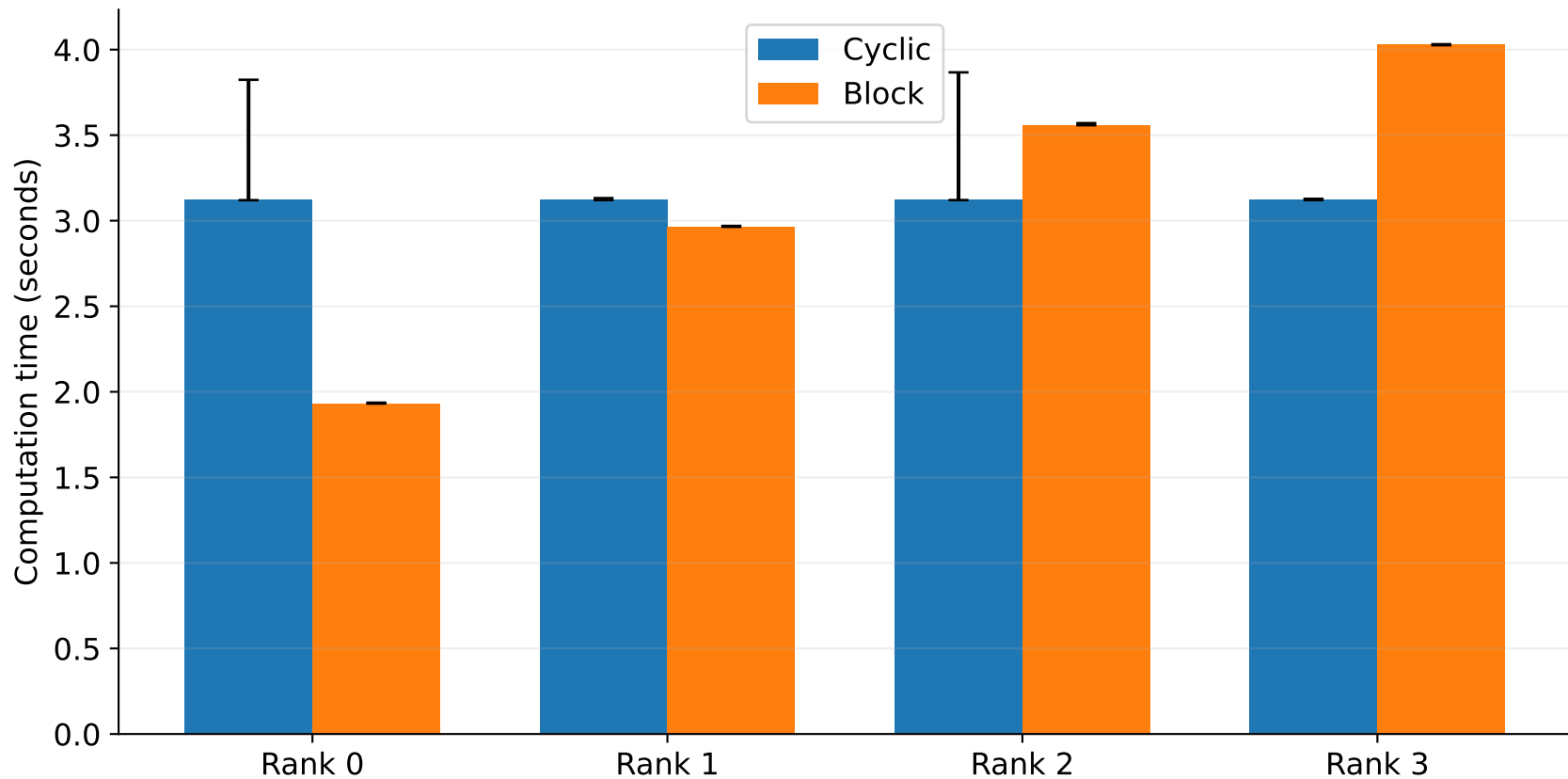
Task 1: computation time by MPI rank
