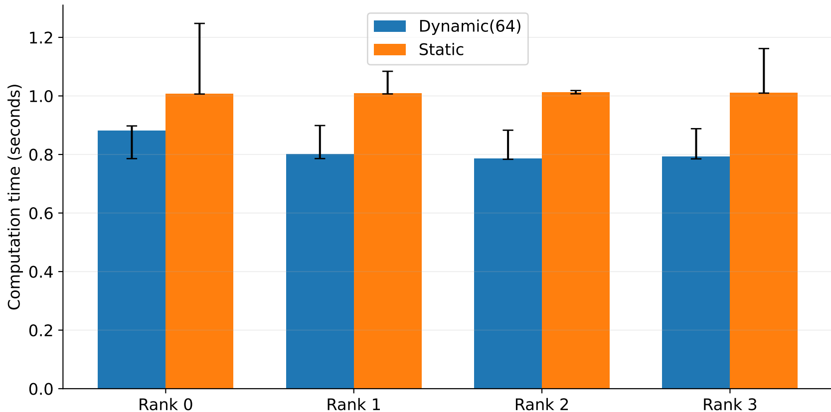
Task 2: computation time by MPI rank
