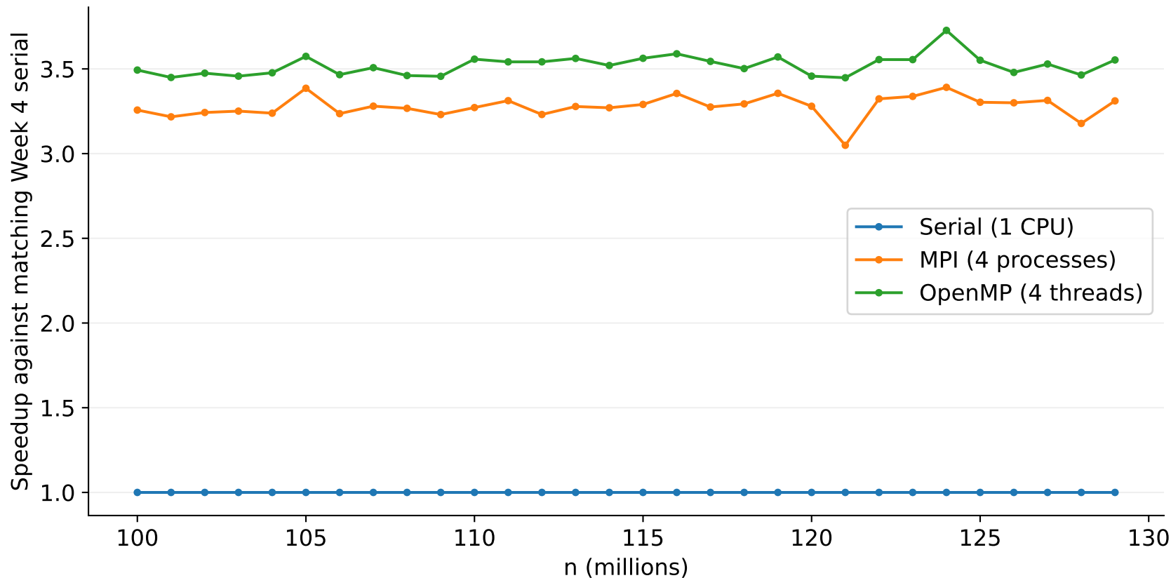
Empirical speedup across 30 input sizes
