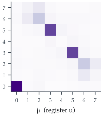
Aer, 4096 shots
