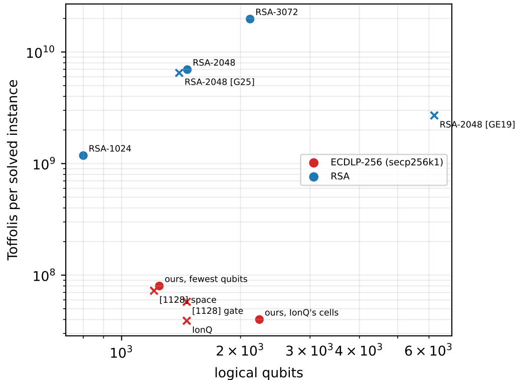
Whole algorithm, logical (o built here, x published)
