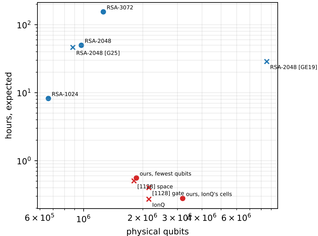
Same, in one surface-code model ( p = 1e-3 , 1 us cycle)
