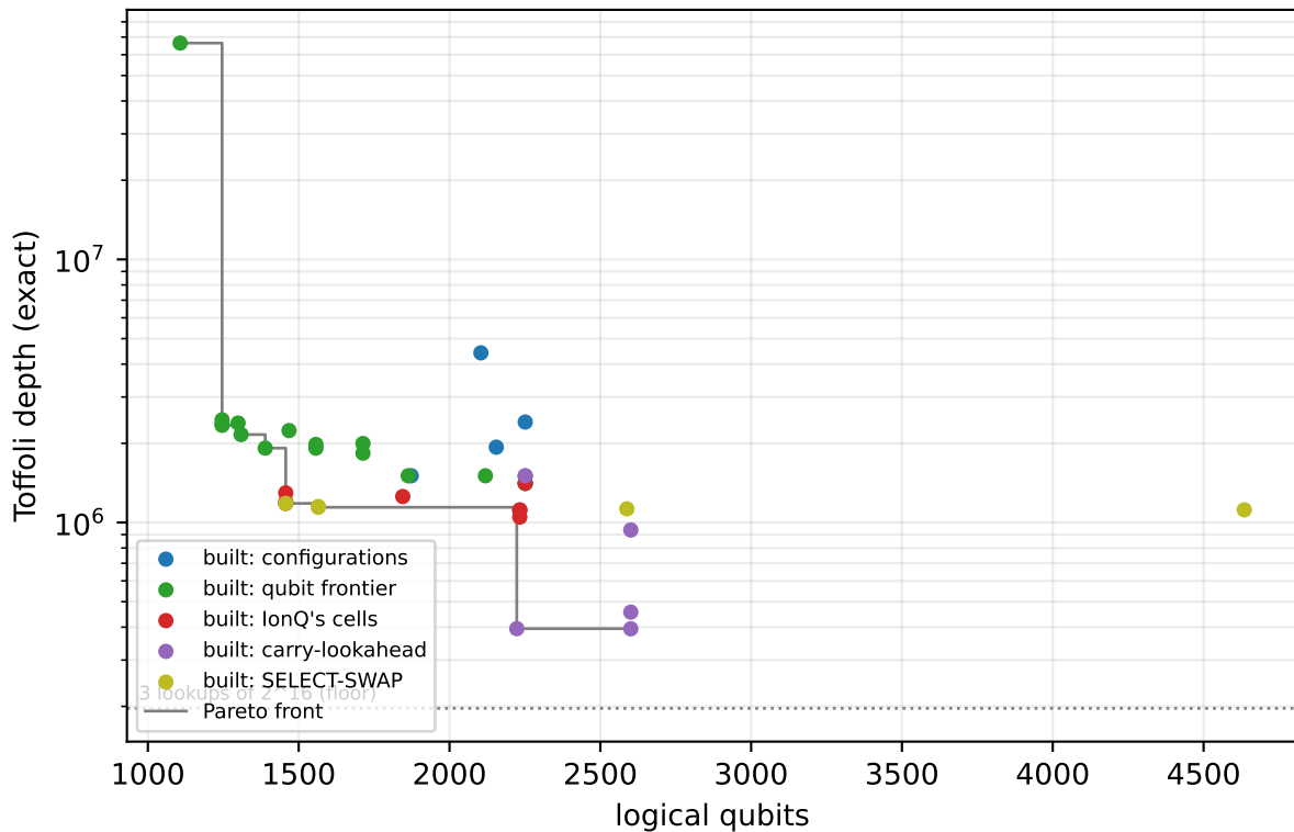
One windowed point addition: qubits against Toffoli depth
