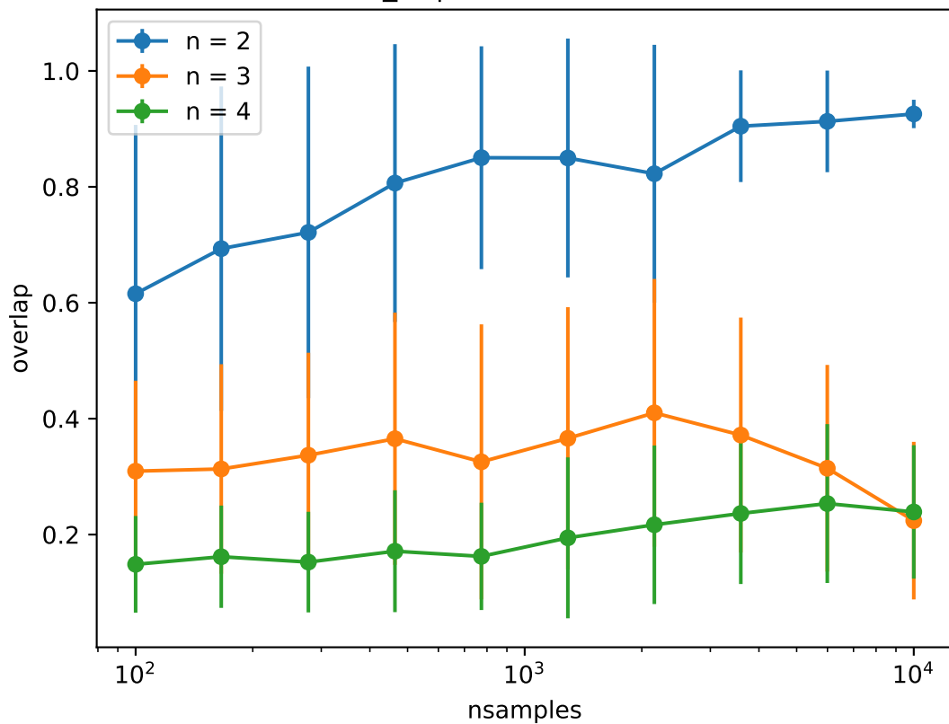
U_W |b^n\rangle with b = 1
