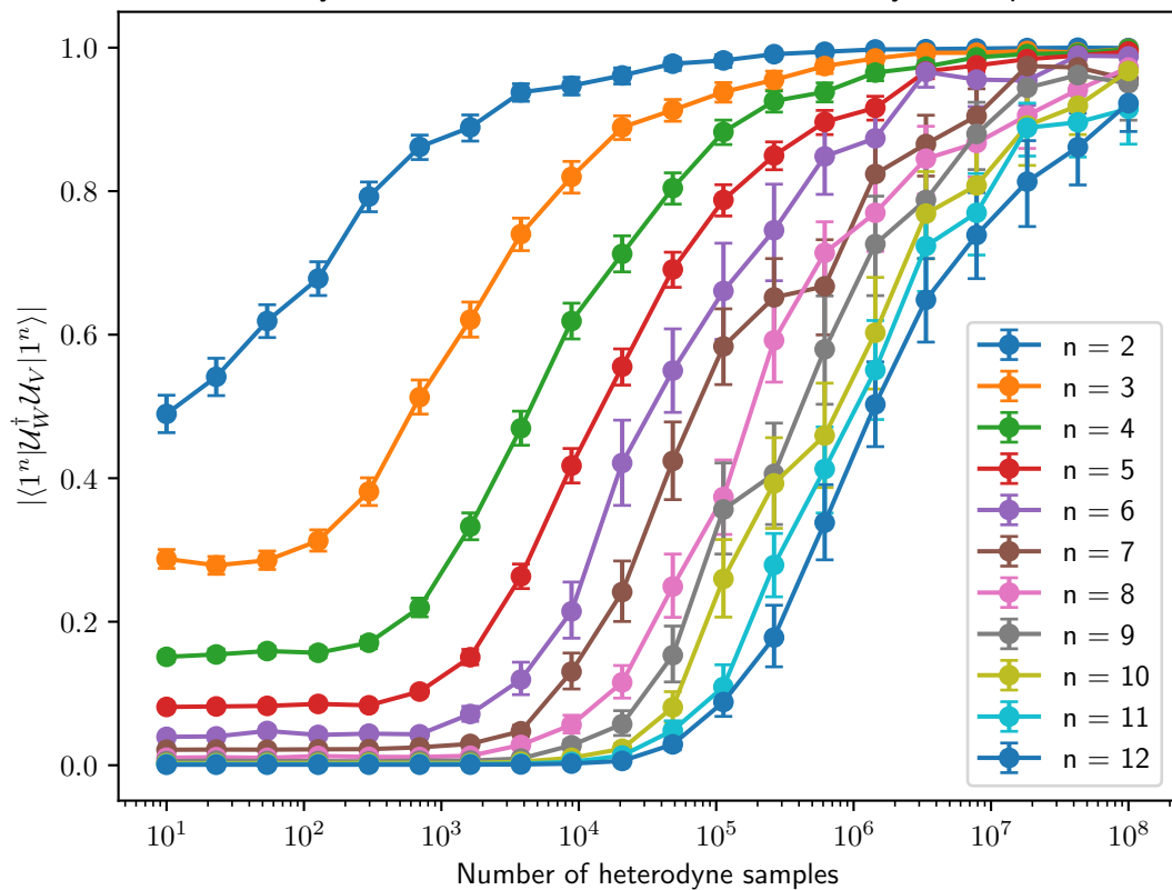
Fidelity of learned state vs number of heterodyne samples
