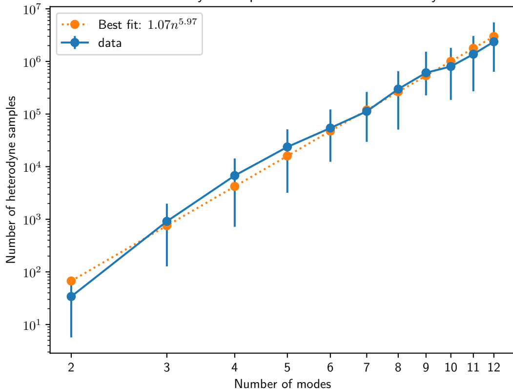
Number of heterodyne samples needed to achieve fidelity = 0.5
