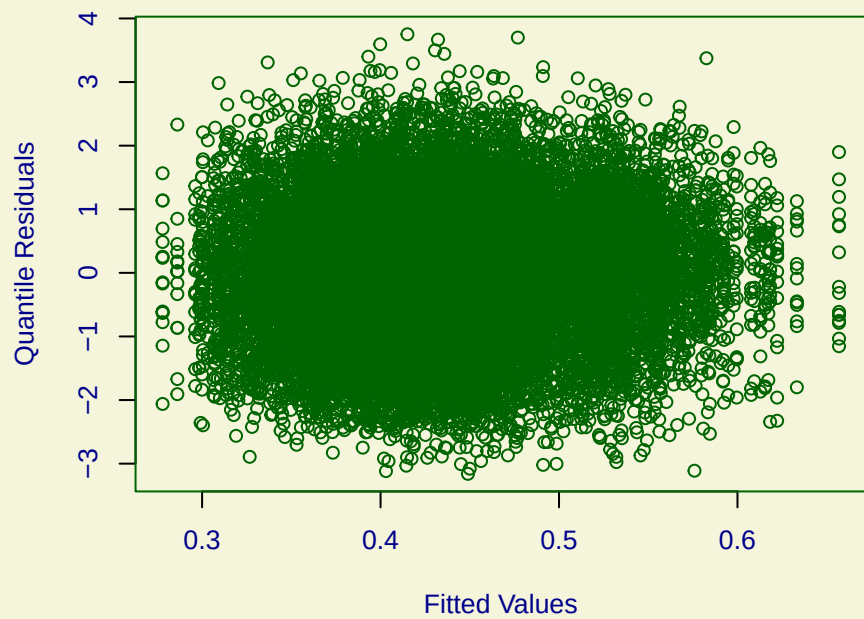
Against Fitted Values
