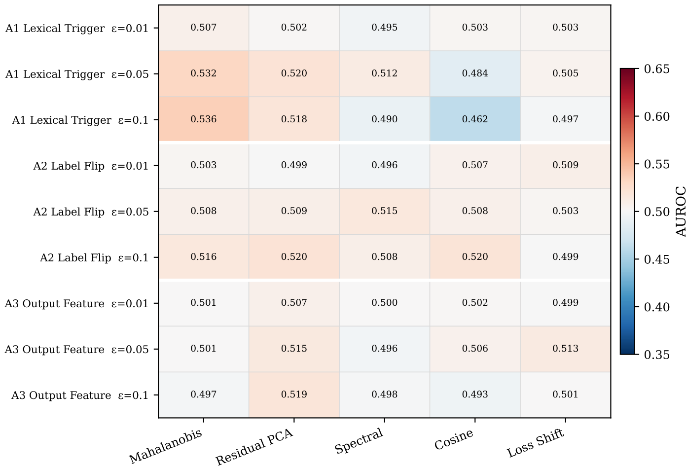
AUROC per attack condition × detection signal
