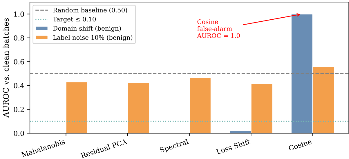
False-alarm control: detection of benign distribution shifts (ideal detector \rightarrow 0.00 for shift, \approx 0.50 for i.i.d. noise)
