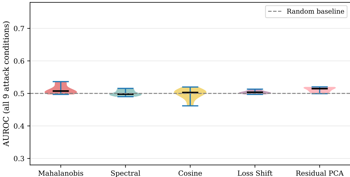
Distribution of AUROC across all attack conditions per detection signal (Qwen2.5-1.5B · LoRA r=8 · HH-RLHF)
