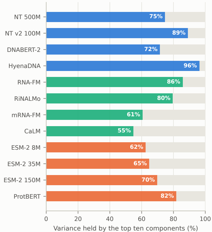
a Variance in the top ten components
