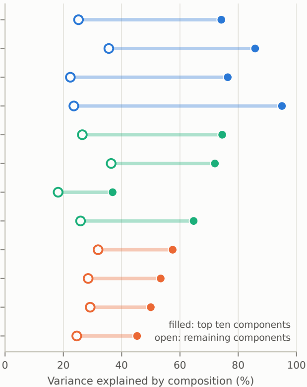
b Composition share: top ten vs rest
