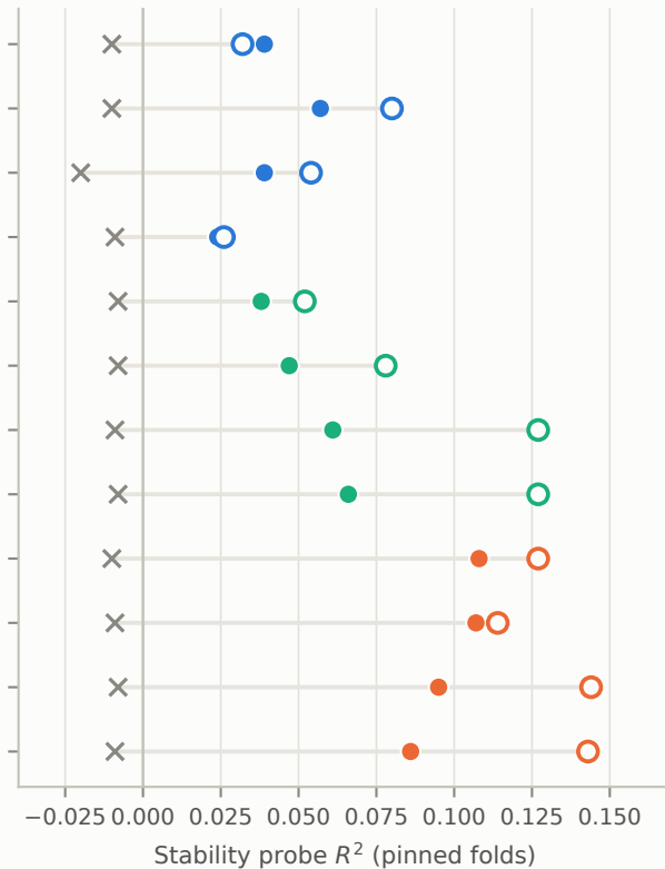
c Where the stability signal sits
