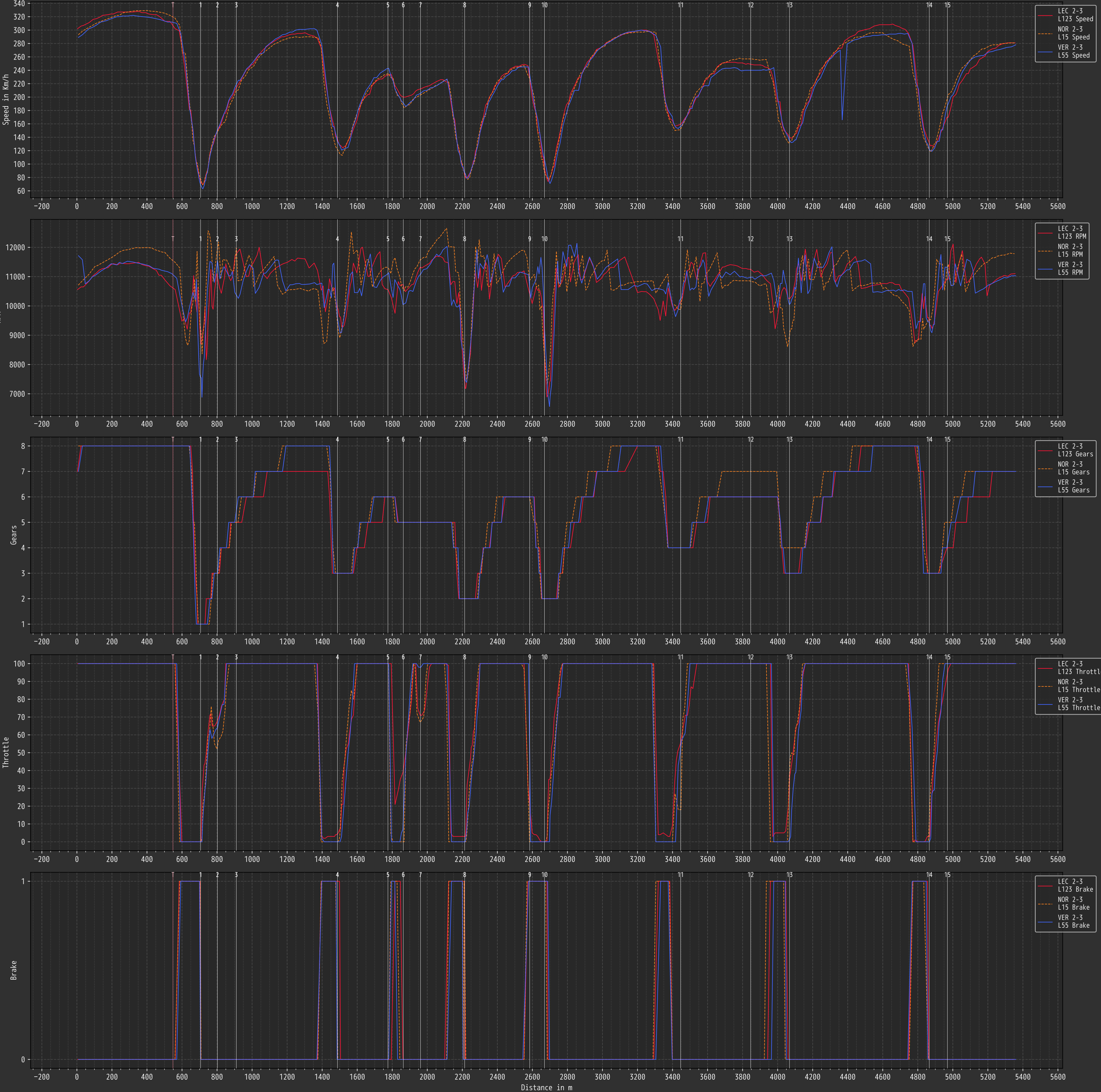
2026 Pre-Season Testing 2-3 Top3 Telemetry overlay
