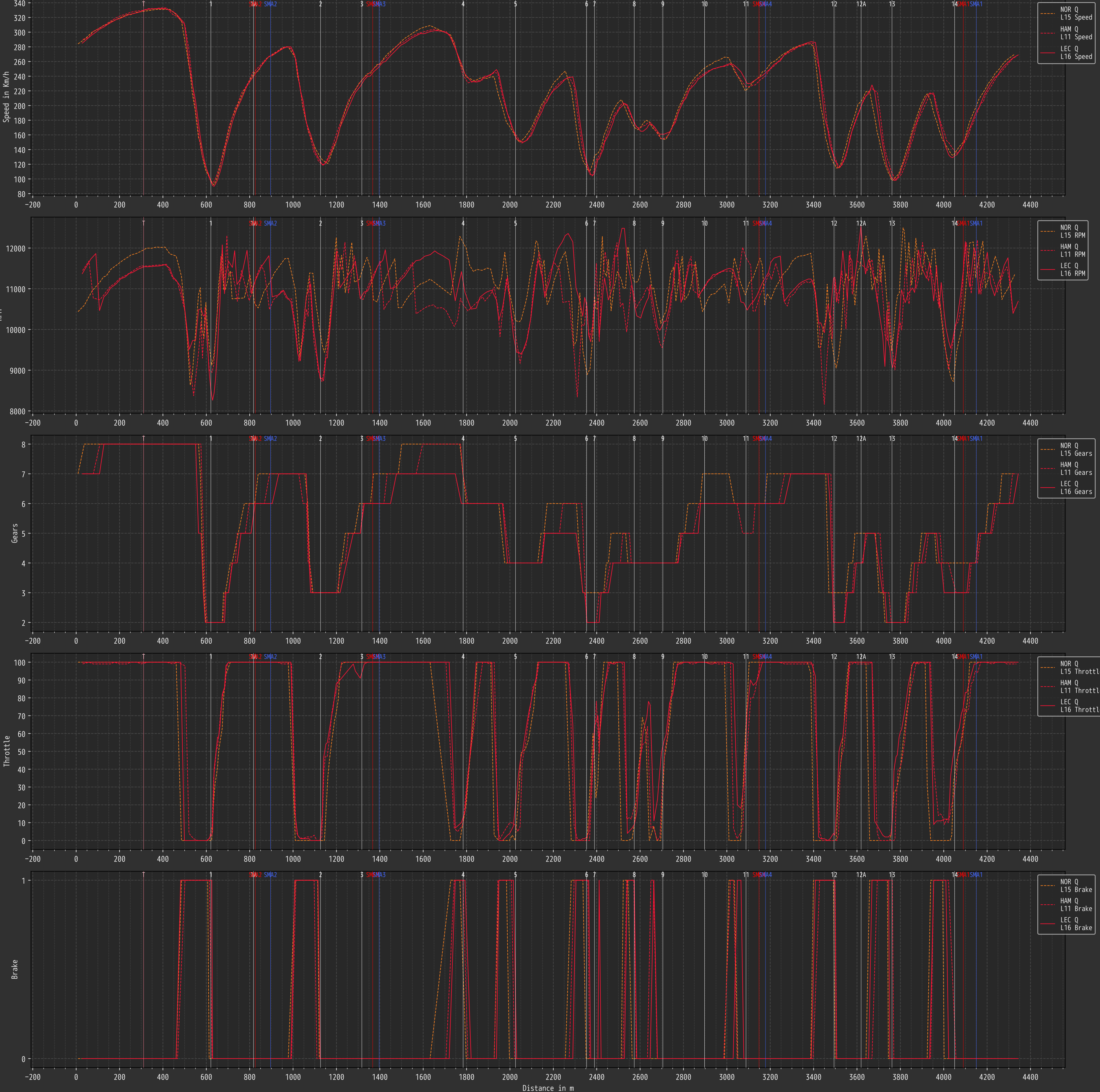
2026 Rd11 Hungarian Grand Prix Qualifying Top3 Telemetry overlay
