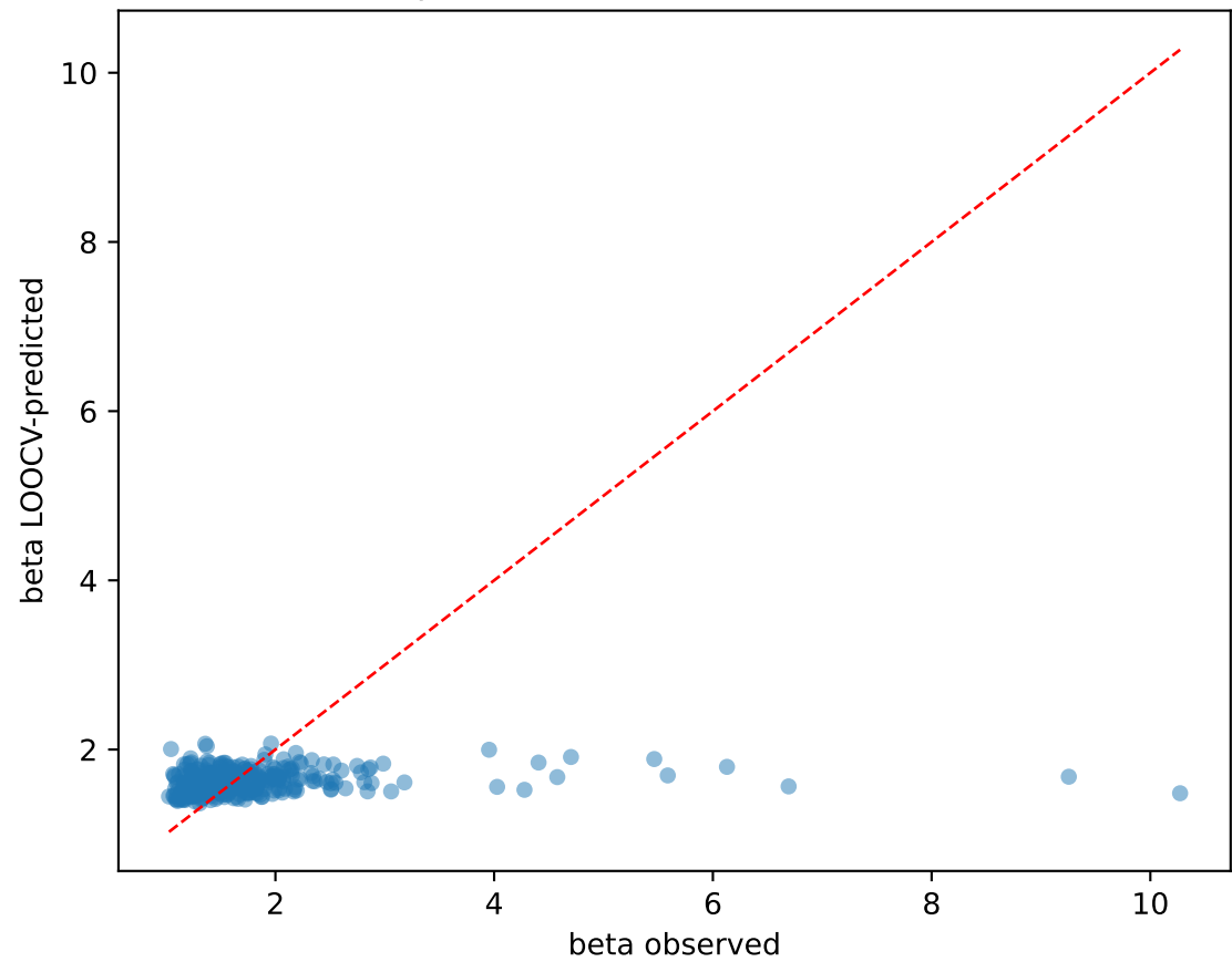
Spatial LOOCV (RMSE = 0.895)
