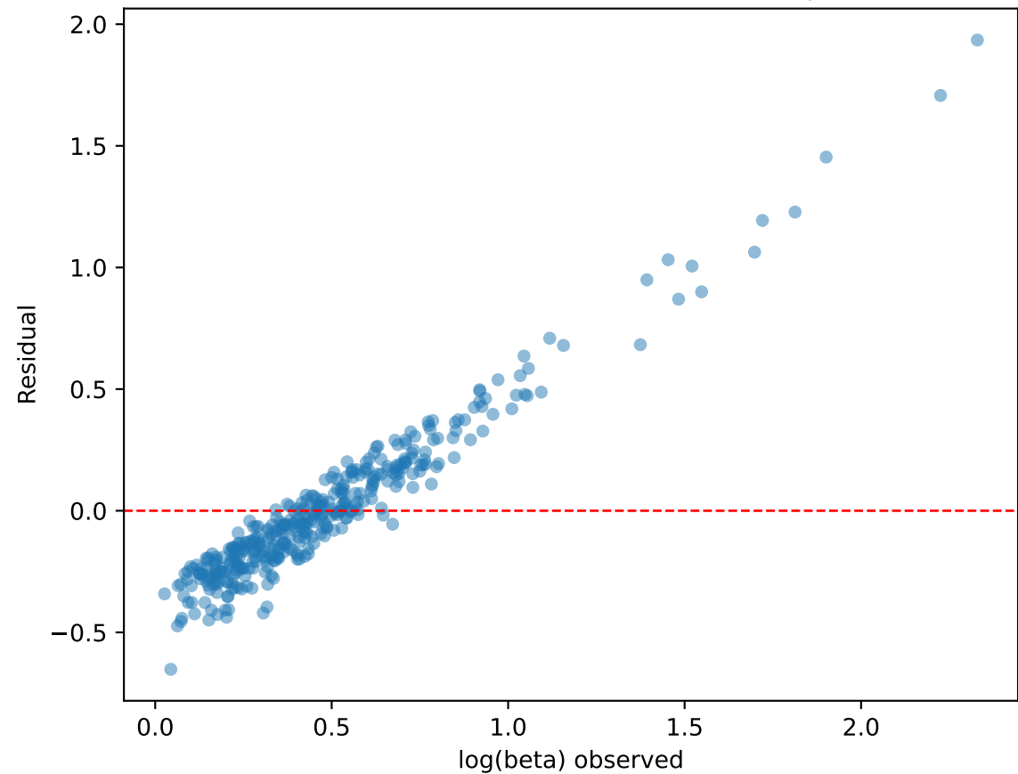
Residuals vs observed (Moran I = -0.044, p=0.051)
