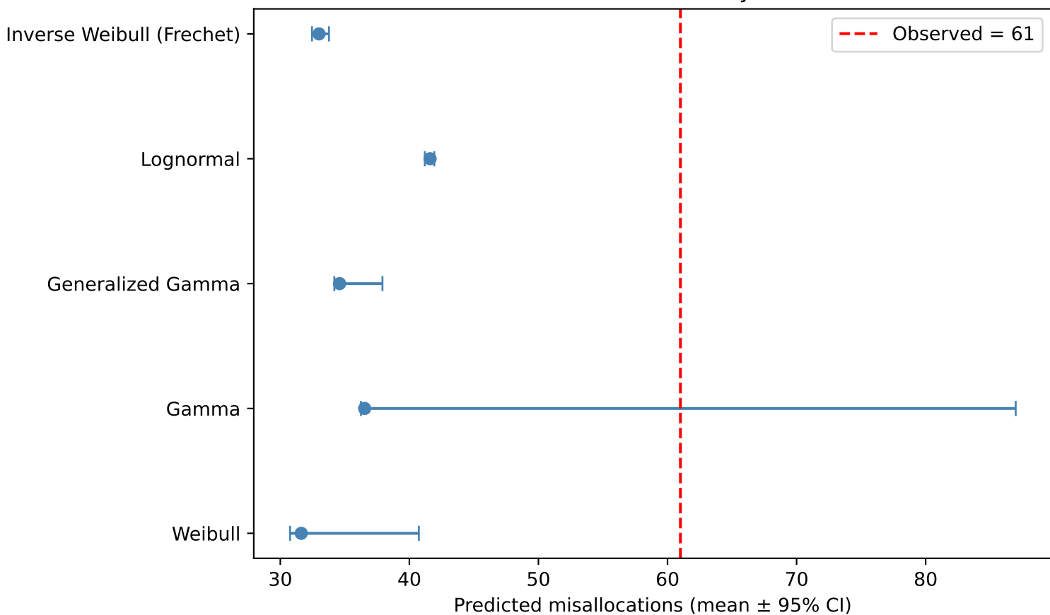
Predicted vs observed misallocations by candidate distribution
