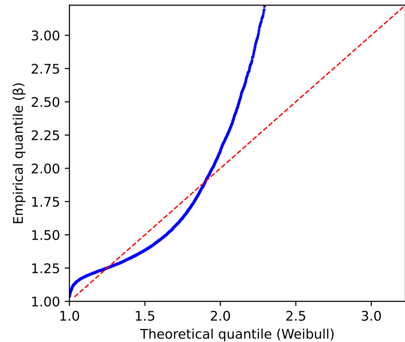
Weibull ( W_1=0.087 )
