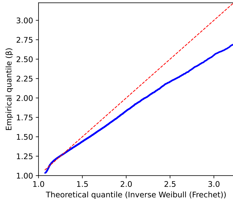
Inverse Weibull (Frechet) ( W_1=0.053 )
