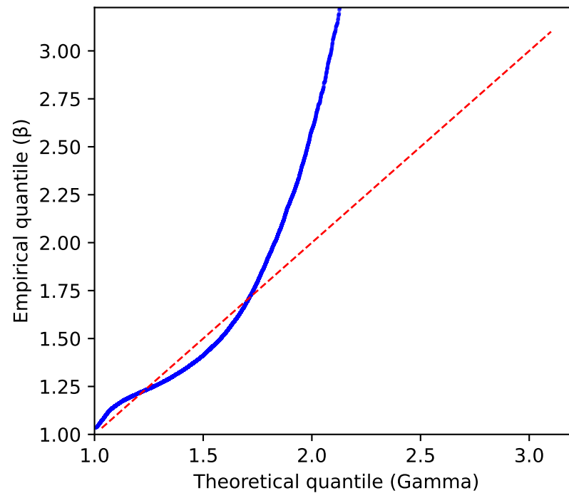
Generalized Gamma ( W_1=0.054 )
