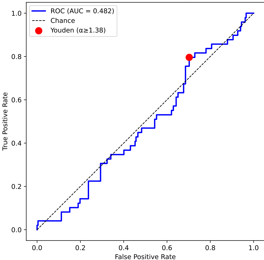
Anisotropy \alpha as misallocation predictor
