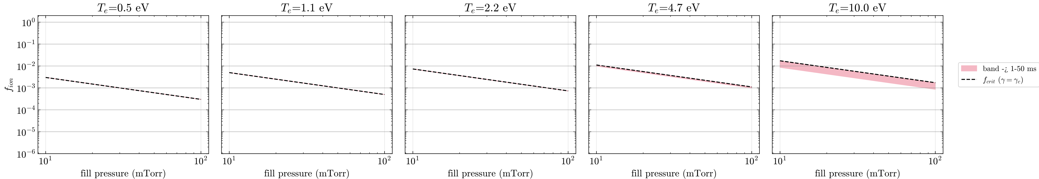
Ionisation fraction at threshold and the narrow band above it giving 1-50 ms (thin gray lines: the 7 requested f_{ion} values)
