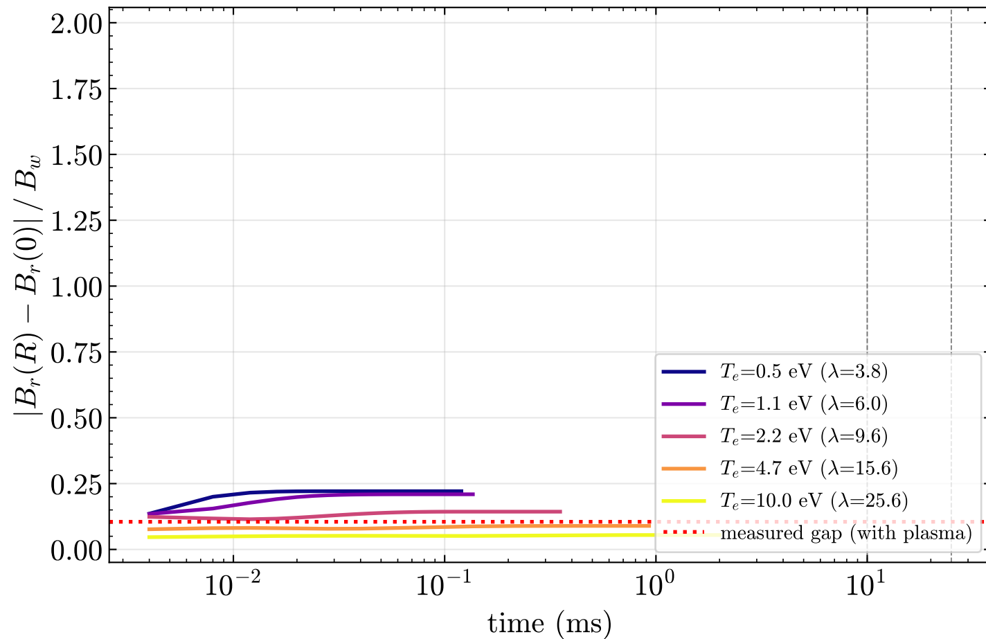
Field-expulsion transient vs. the observed 10 ms / 25 ms marks (dashed vertical: 10, 25 ms; dotted red: measured (1.6-1.0) \text{ G} / 6 \text{ G} = 0.11 )
