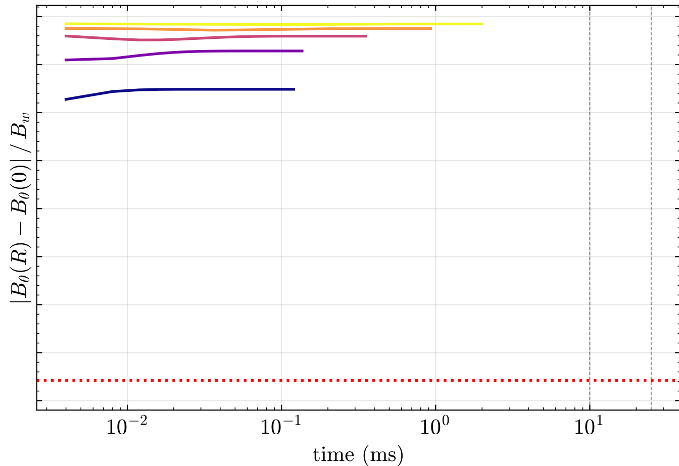
Field-expulsion transient vs. the observed 10 ms / 25 ms marks (dashed vertical: 10, 25 ms; dotted red: measured (1.6-1.0) \text{ G} / 6 \text{ G} = 0.11 )
