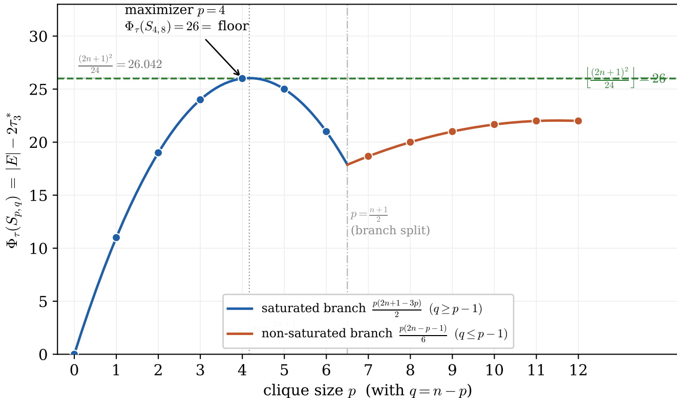
\Phi_\tau on complete-split graphs S_{p,q} , p+q=n=12
