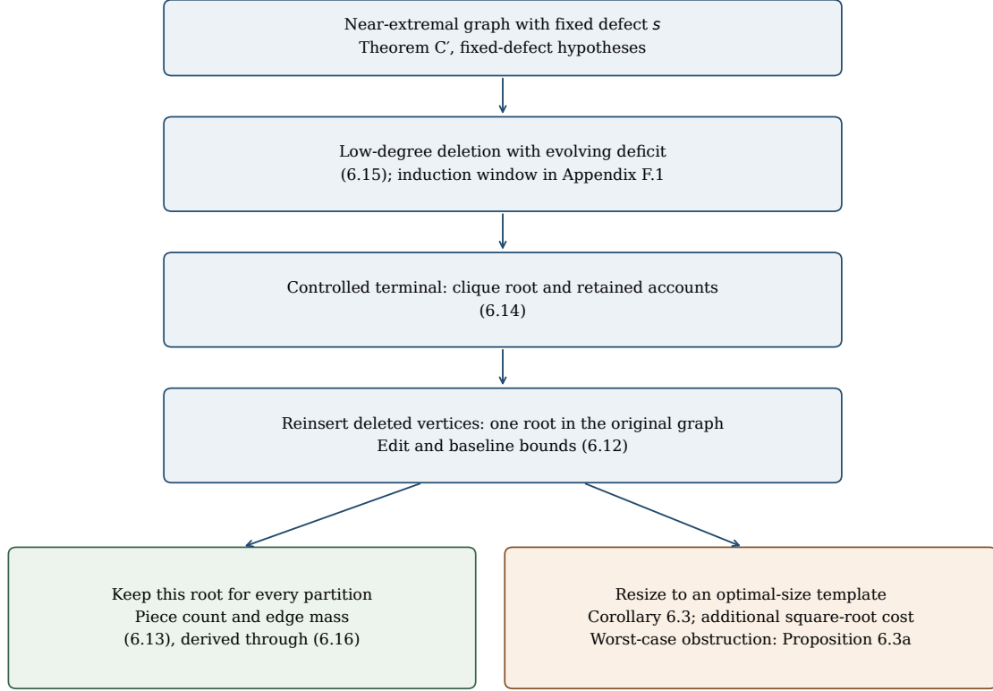
Figure 3: Proof structure for fixed-defect same-root stability. Theorem C': low-degree deletion reaches the controlled terminal, and reinsertion transports its root back to the original graph. The retained accounts then control every partition on that same root. Resizing to an optimal template is a separate step (Corollary 6.3), with the square-root cost illustrated by Proposition 6.3a. The diagram is schematic; Appendix F.1 supplies the induction window.
