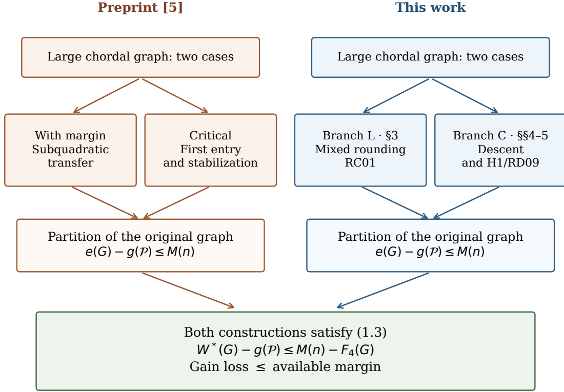
Figure 4: Comparison of mechanisms. Preprint [5] and this work separate two alternative cases and construct a partition satisfying (1.3). Arrows indicate implications toward the conclusion, not passage from one regime to the other. The source locations for the left column are given in Section 8.
